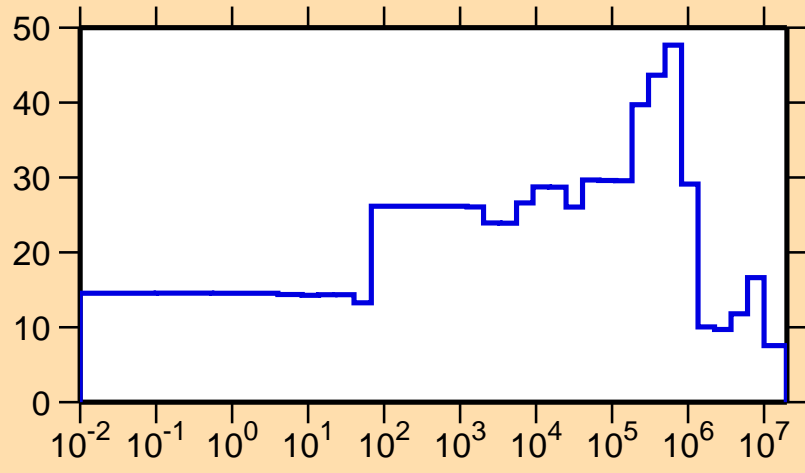
\Delta\sigma/\sigma vs. E for ^{255}\text{Md}(n,\text{el.})
