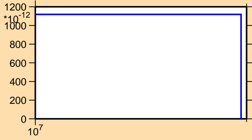
\sigma vs. E for ^{255}\text{Md}(n,2np)
