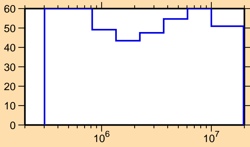
\Delta\sigma/\sigma vs. E for ^{255}\text{Md}(n,n\text{cont.})
