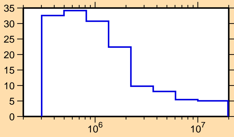
\Delta\sigma/\sigma vs. E for ^{255}\text{Md}(n,n\text{onel.})
