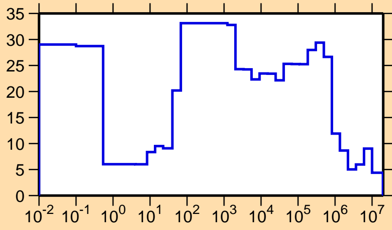
\Delta\sigma/\sigma vs. E for ^{255}\text{Md}(n,\text{tot.})
