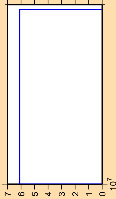
\Delta\sigma/\sigma vs. E for ^{255}\text{Md}(\text{mt117})
