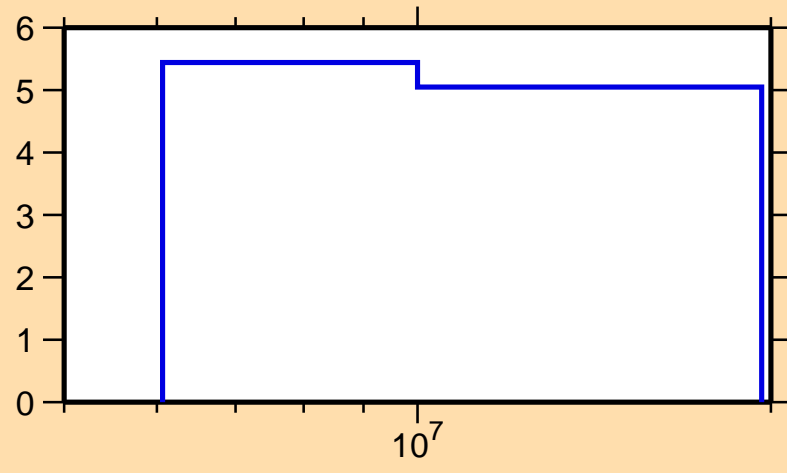
\Delta\sigma/\sigma vs. E for ^{255}\text{Md}(n,\text{nonel.})
