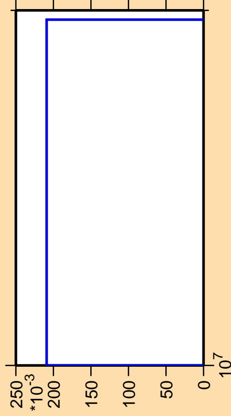
\Delta\sigma/\sigma vs. E for ^{255}\text{Md} (mt 45)
