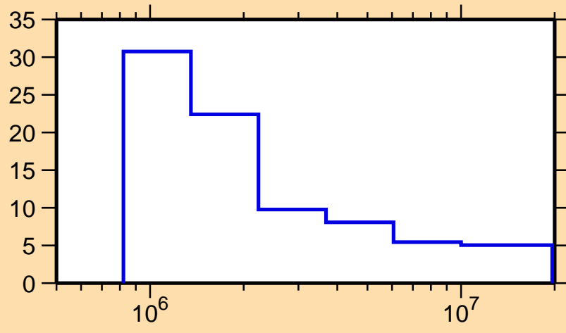
\Delta\sigma/\sigma vs. E for ^{255}\text{Md}(n,\text{nonel.})
