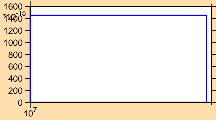
\sigma vs. E for ^{255}\text{Md}(\text{mt117})
