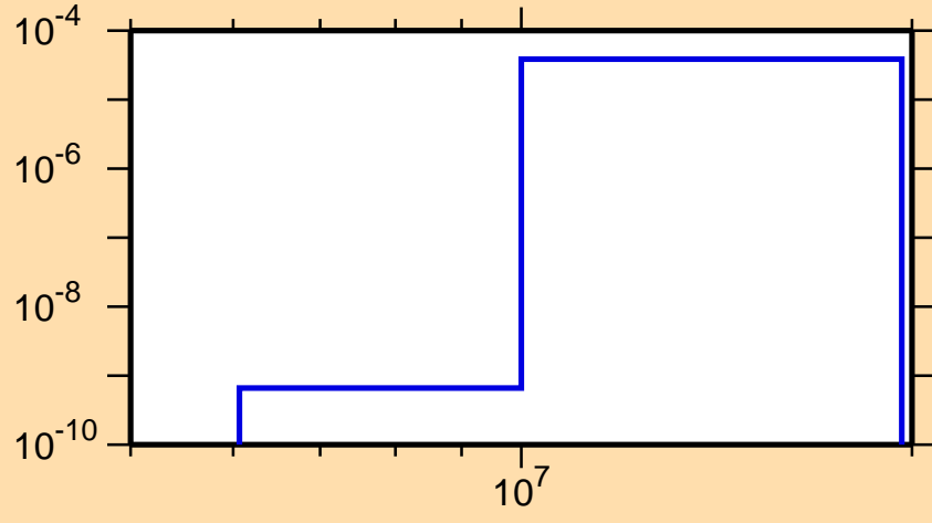
\sigma vs. E for ^{255}\text{Md}(n,np)
