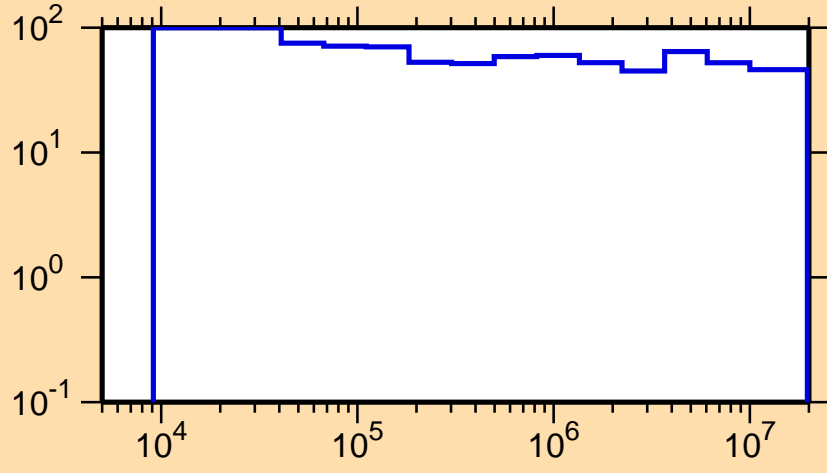
\Delta\sigma/\sigma vs. E for ^{255}\text{Md}(n,n_1)
