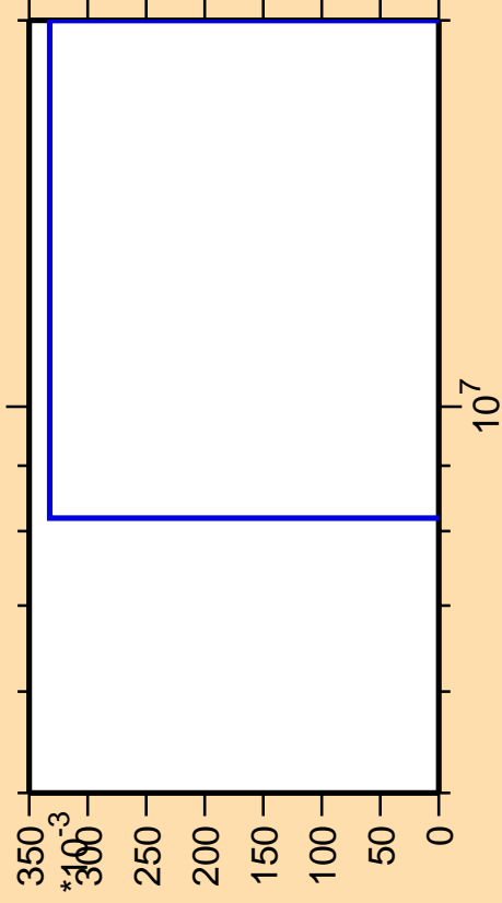
\Delta\sigma/\sigma vs. E for ^{255}\text{Md}(n,3n\alpha)
