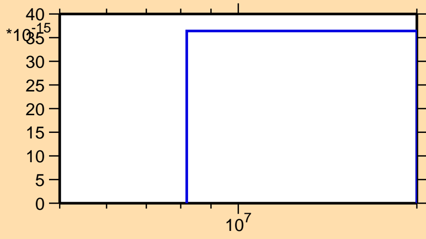
\sigma vs. E for ^{255}\text{Md} (mt 45)
