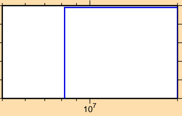
\sigma vs. E for ^{255}\text{Md}(n,nd)
