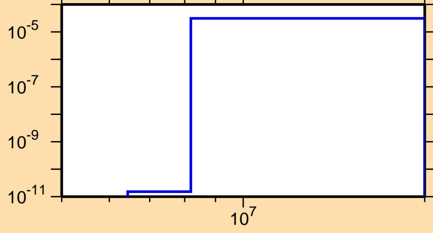
\sigma vs. E for ^{255}\text{Md}(n,np)
