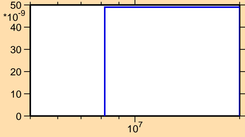
\sigma vs. E for ^{255}\text{Md}(n,nd)
