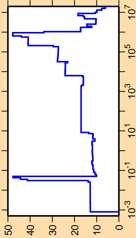
\Delta\sigma/\sigma vs. E for ^{256}\text{Md}(n,\text{el.})
