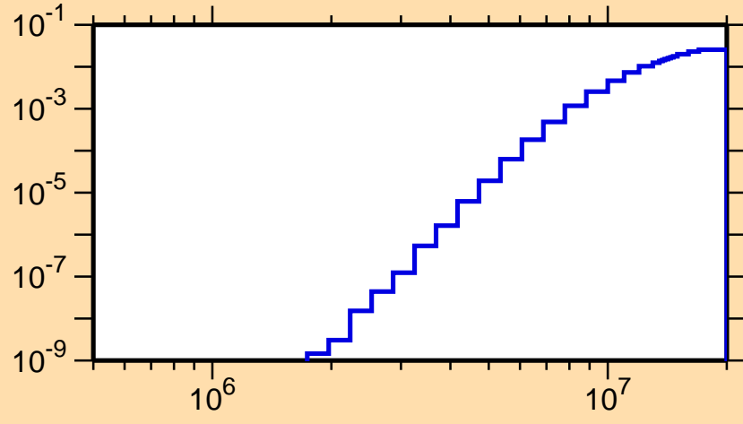
\sigma vs. E for ^{256}\text{Md}(n,p)
