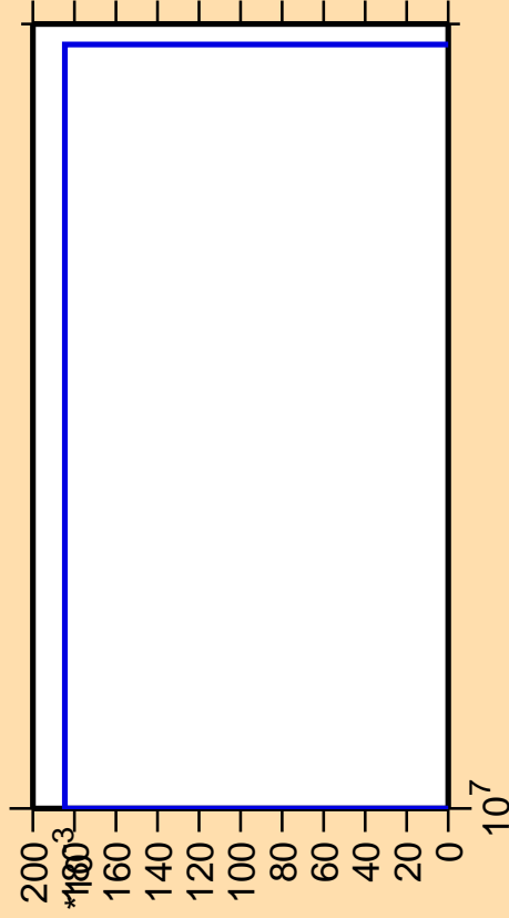
\Delta\sigma/\sigma vs. E for ^{256}\text{Md}(n,3n\alpha)
