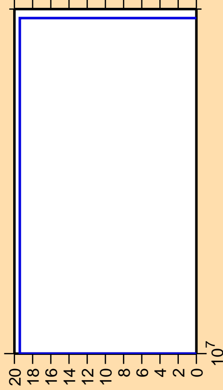
\Delta\sigma/\sigma vs. E for ^{256}\text{Md}(n,p\alpha)
