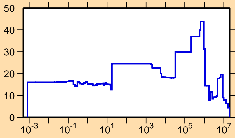
\Delta\sigma/\sigma vs. E for ^{257}\text{Md}(n,el.)
