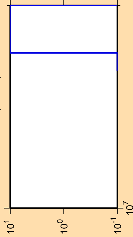
\Delta\sigma/\sigma vs. E for ^{257}\text{Md} (mt 11)
