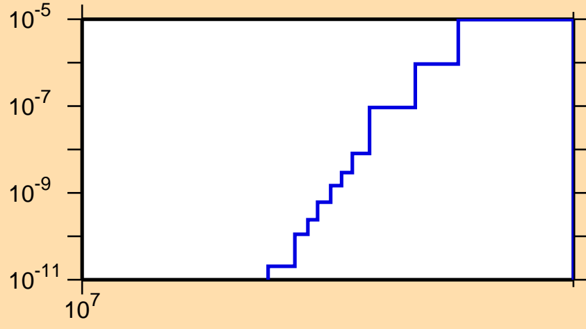
\sigma vs. E for ^{257}\text{Md}(n,\text{nd})
