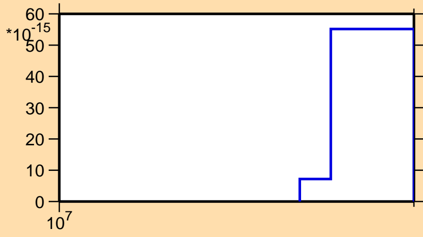
\sigma vs. E for ^{257}\text{Md}(n,p\alpha)
