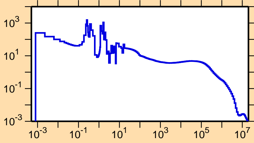
\sigma vs. E for ^{257}\text{Md}(n,\gamma)
