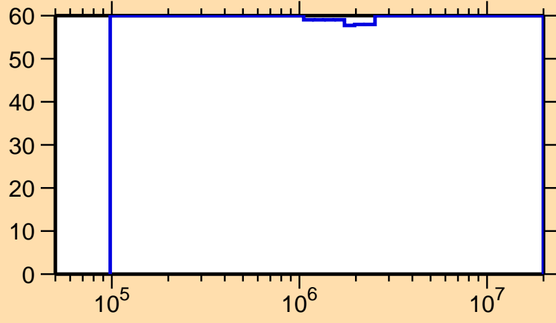
\Delta\sigma/\sigma vs. E for ^{257}\text{Md}(n,ncont.)
