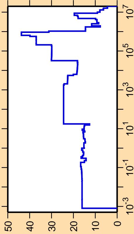
\Delta\sigma/\sigma vs. E for ^{257}\text{Md}(n,\text{el.})
