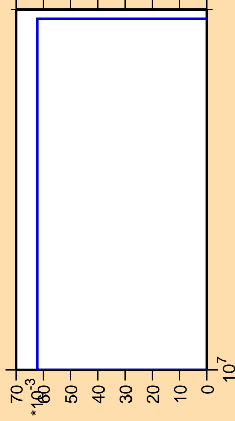
\Delta\sigma/\sigma vs. E for ^{257}\text{Md} (mt 11)
