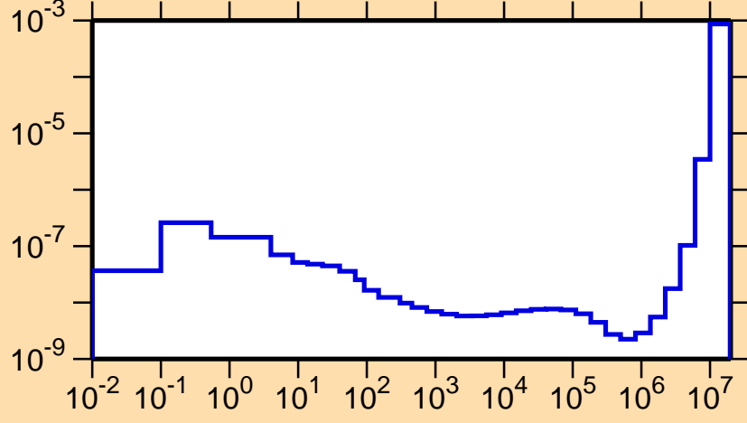
\sigma vs. E for ^{257}\text{Md}(n,\alpha)
