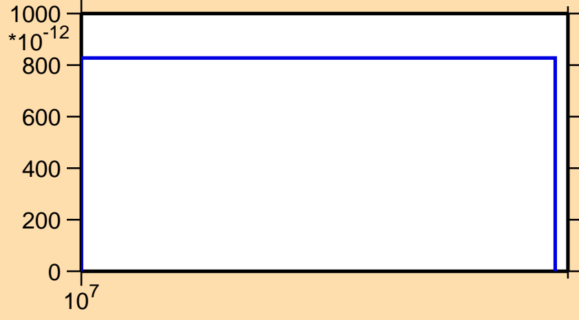
\sigma vs. E for ^{257}\text{Md}(n,2np)
