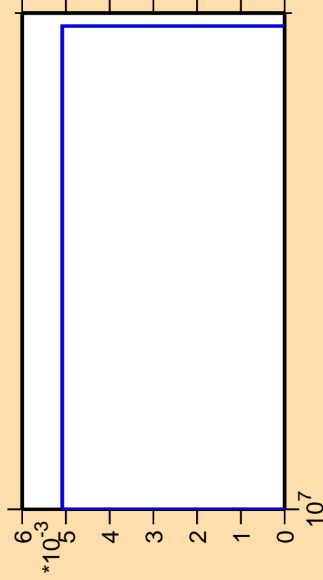
\Delta\sigma/\sigma vs. E for ^{257}\text{Md}(n,p\alpha)
