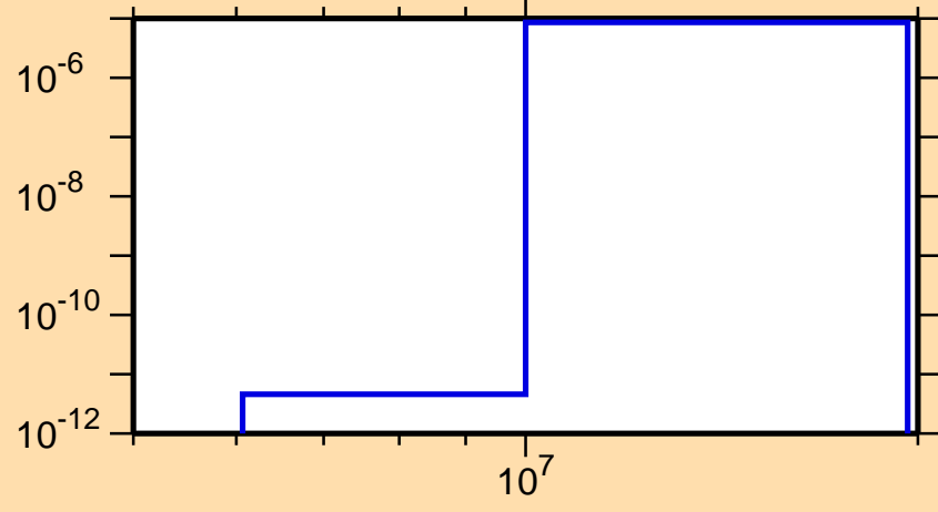
\sigma vs. E for ^{257}\text{Md}(n,np)
