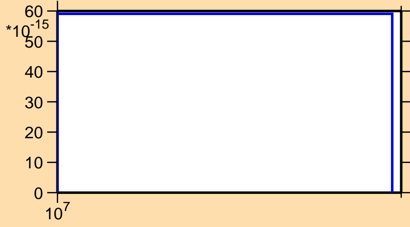
\sigma vs. E for ^{257}\text{Md} (mt 11)
