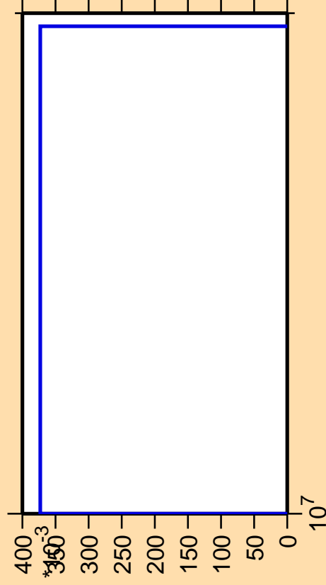
\Delta\sigma/\sigma vs. E for ^{257}\text{Md}(n,\text{He3})
