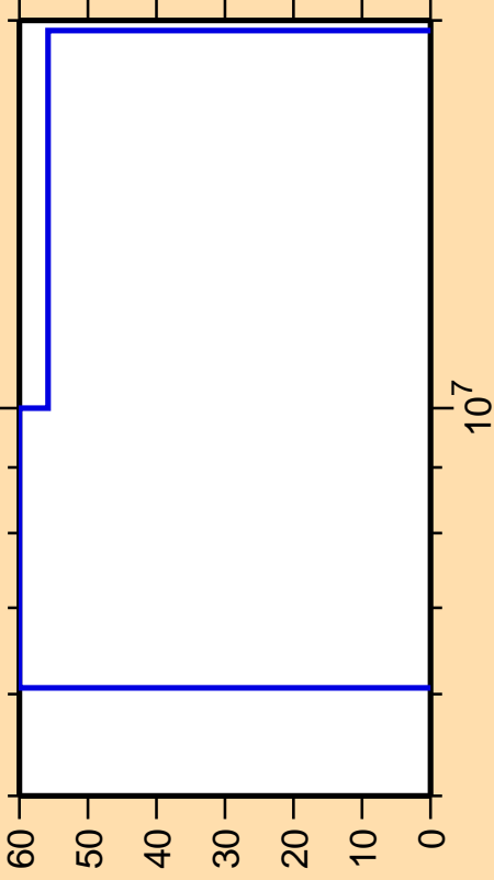
\Delta\sigma/\sigma vs. E for ^{257}\text{Md}(n,2n)
