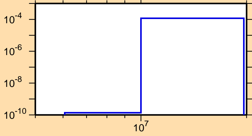
\sigma vs. E for ^{257}\text{Md}(n,t)
