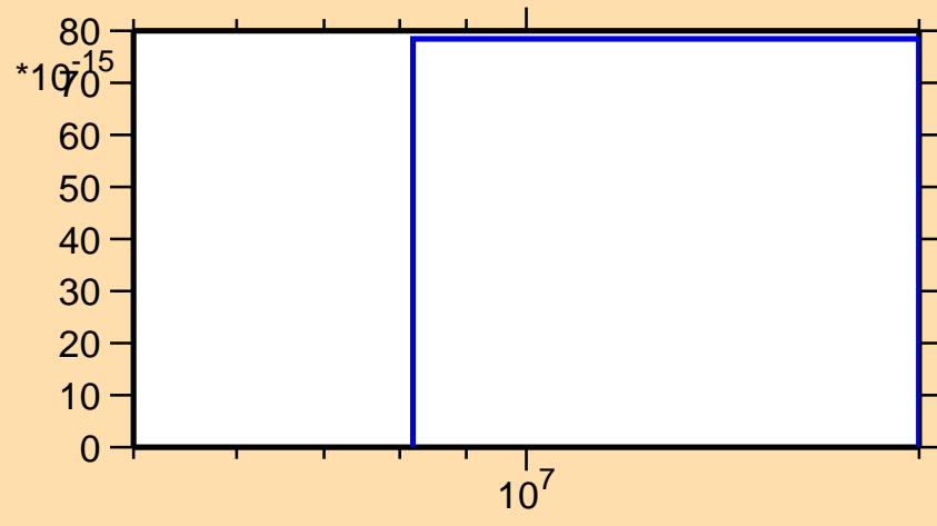
\sigma vs. E for ^{257}\text{Md}(\text{mt } 11)
