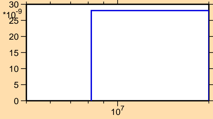
\sigma vs. E for ^{257}\text{Md}(n,2n\alpha)
