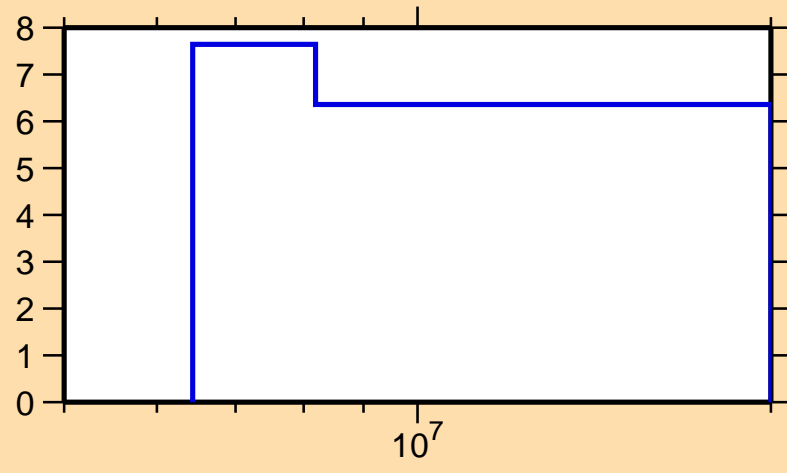
\Delta\sigma/\sigma vs. E for ^{257}\text{Md}(n,\text{nonel.})
