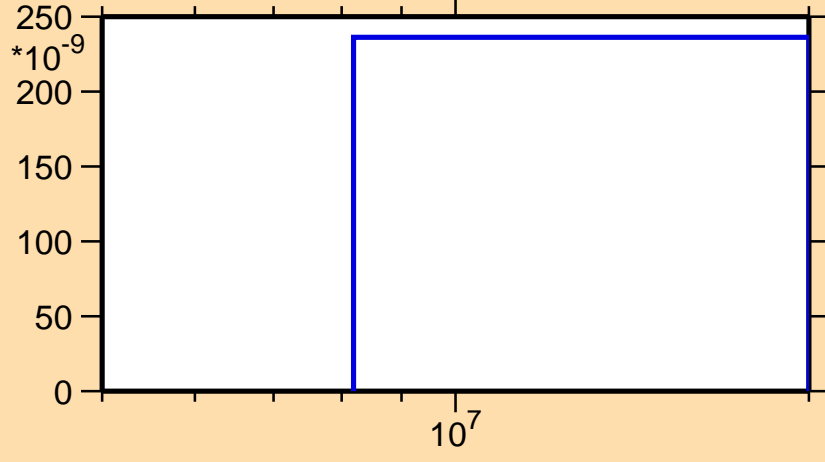
\sigma vs. E for ^{257}\text{Md}(n,nt)
