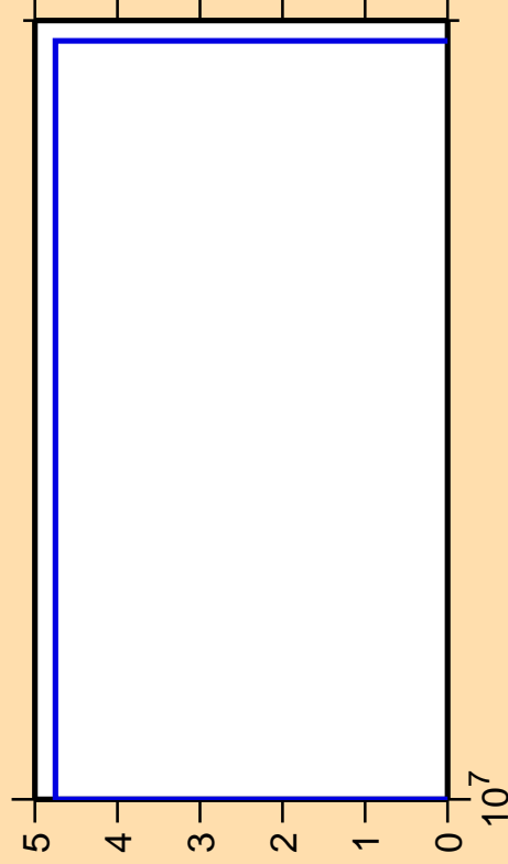
\Delta\sigma/\sigma vs. E for ^{258}\text{Md}(n,\text{He3})
