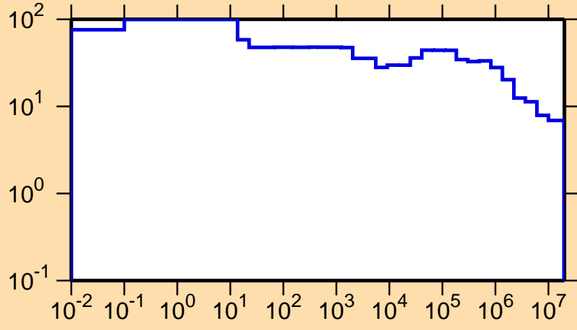
\Delta\sigma/\sigma vs. E for ^{258}\text{Md}(n,\text{nonel.})
