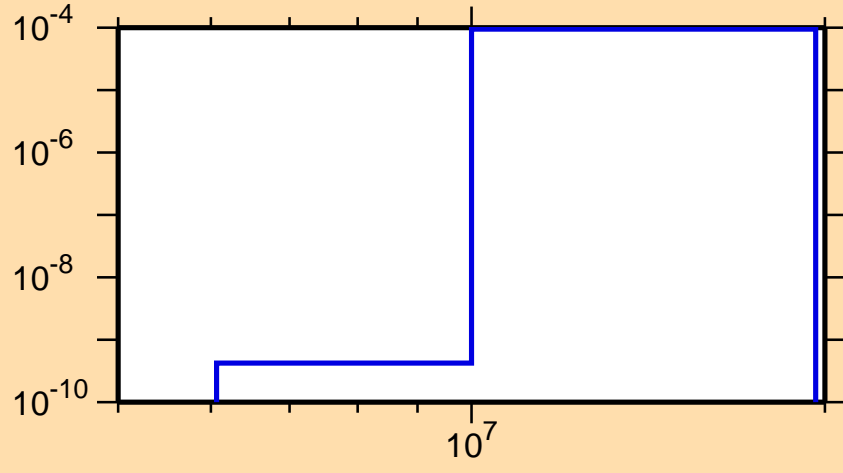
\sigma vs. E for ^{258}\text{Md}(n,d)
