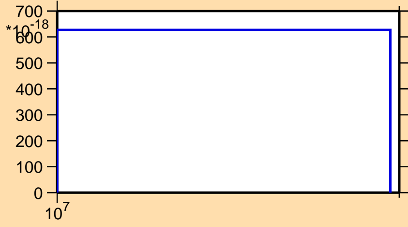
\sigma vs. E for ^{258}\text{Md}(\text{mt } 11)
