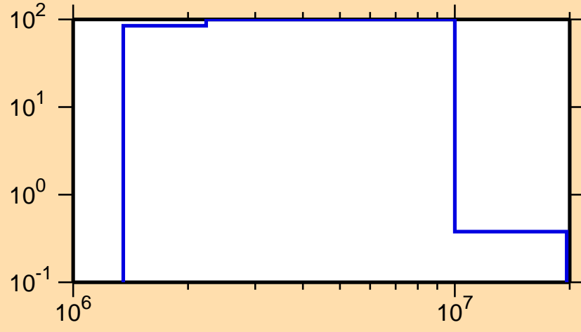
\Delta\sigma/\sigma vs. E for ^{258}\text{Md}(n,n_1)
