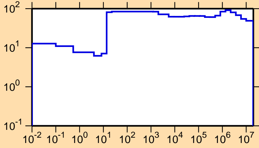
\Delta\sigma/\sigma vs. E for ^{258}\text{Md}(n,f)
