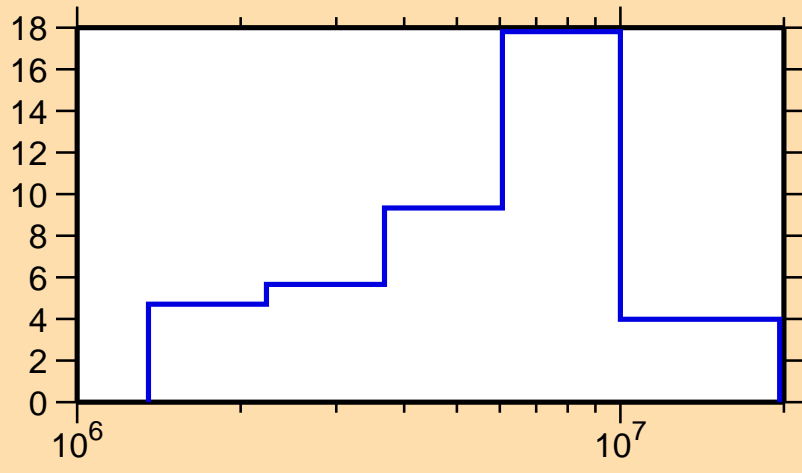
\Delta\sigma/\sigma vs. E for ^{258}\text{Md}(n,\text{el.})
