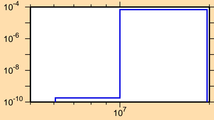
\sigma vs. E for ^{258}\text{Md}(n,t)
