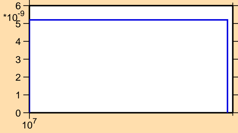
\sigma vs. E for ^{258}\text{Md}(n,2np)
