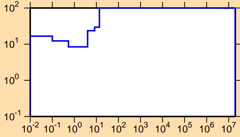
\Delta\sigma/\sigma vs. E for ^{258}\text{Md}(n,\gamma)
