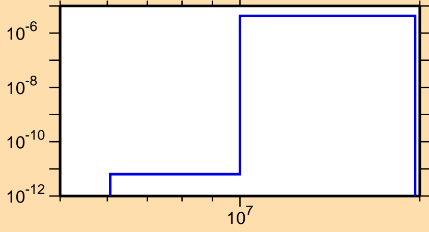
\sigma vs. E for ^{258}\text{Md}(n,np)
