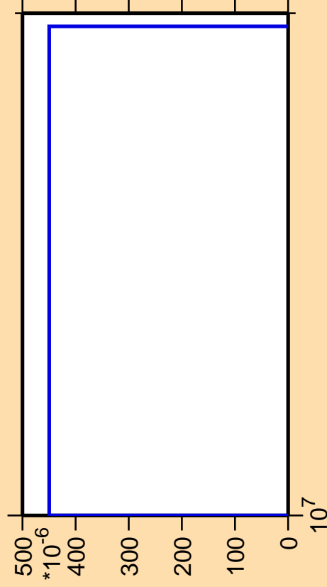
\Delta\sigma/\sigma vs. E for ^{258}\text{Md}(\text{mt } 11)
