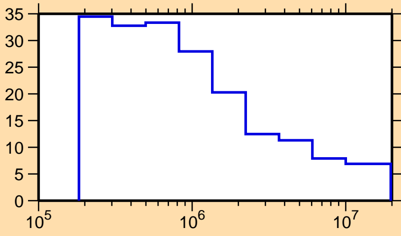
\Delta\sigma/\sigma vs. E for ^{258}\text{Md}(n,\text{nonel.})
