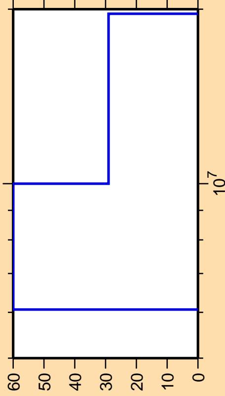
\Delta\sigma/\sigma vs. E for ^{258}\text{Md}(n,t)
