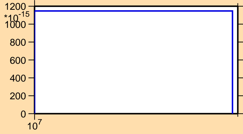
\sigma vs. E for ^{258}\text{Md}(n,\text{He3})
