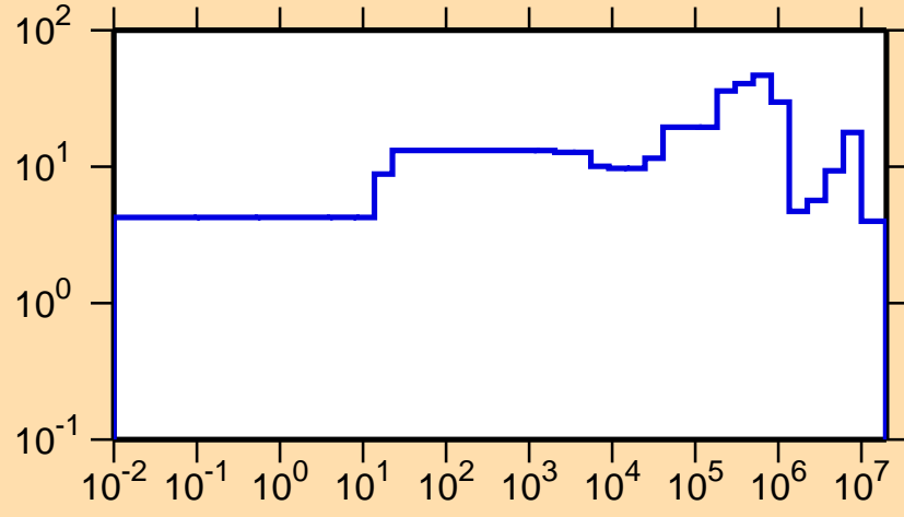
\Delta\sigma/\sigma vs. E for ^{258}\text{Md}(n,\text{el.})
