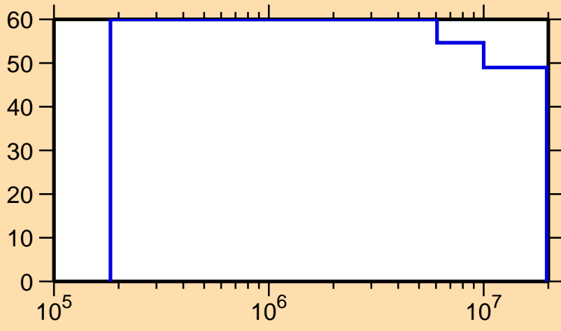
\Delta\sigma/\sigma vs. E for ^{258}\text{Md}(n,f)
