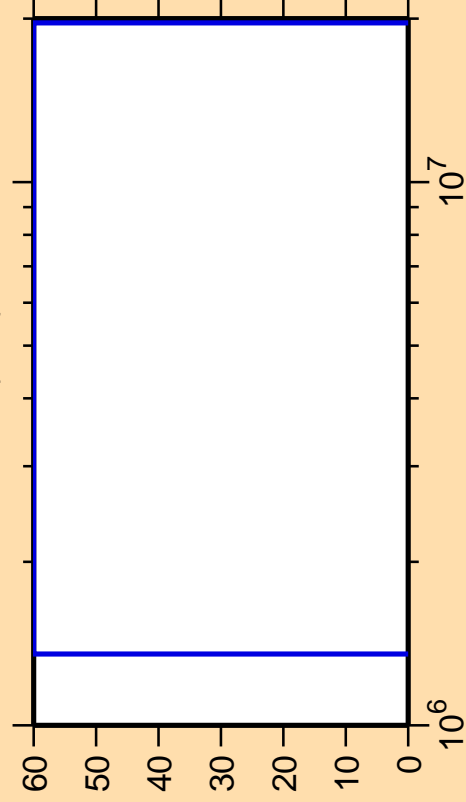
\Delta\sigma/\sigma vs. E for ^{258}\text{Md}(n,\alpha)
