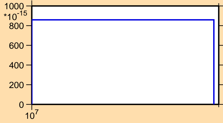
\sigma vs. E for ^{258}\text{Md}(n,3n\alpha)
