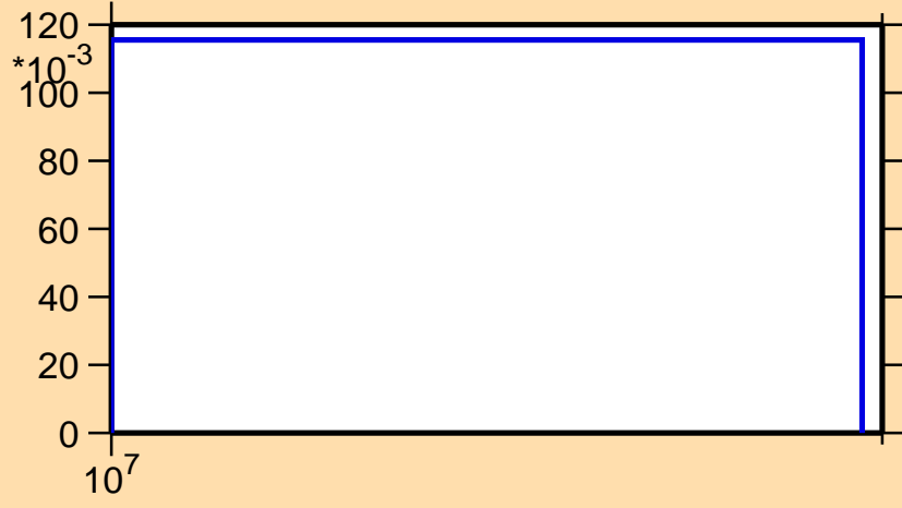
\sigma vs. E for ^{258}\text{Md}(n,3n)
