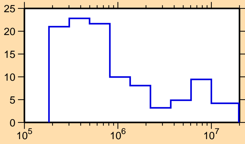
\Delta\sigma/\sigma vs. E for ^{258}\text{Md}(n,\text{tot.})
