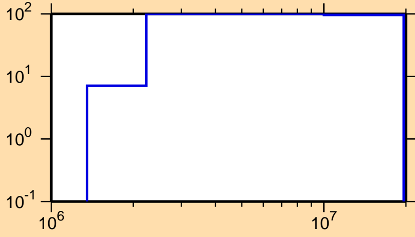
\Delta\sigma/\sigma vs. E for ^{258}\text{Md}(n,p)
