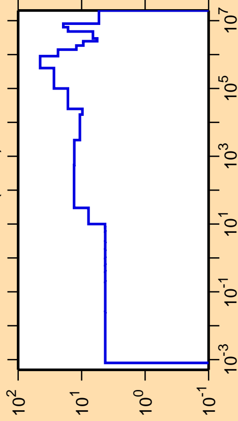
\Delta\sigma/\sigma vs. E for ^{258}\text{Md}(n,\text{el.})
