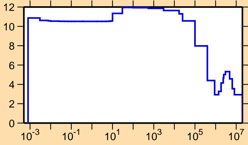
\sigma vs. E for ^{258}\text{Md}(n,\text{el.})
