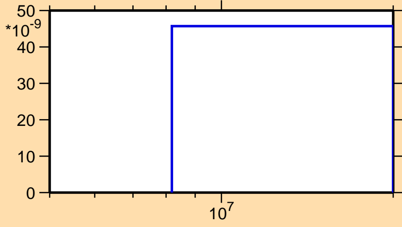
\sigma vs. E for ^{258}\text{Md}(n,nd)
