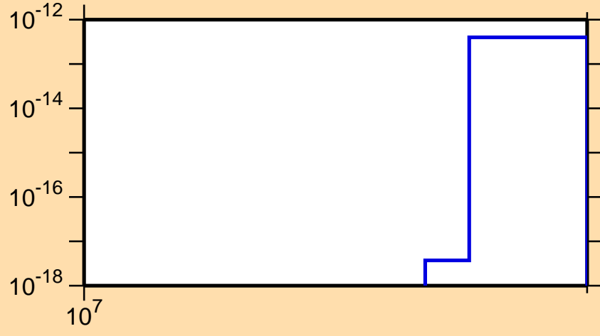
\sigma vs. E for ^{258}\text{Md} (mt 11)
