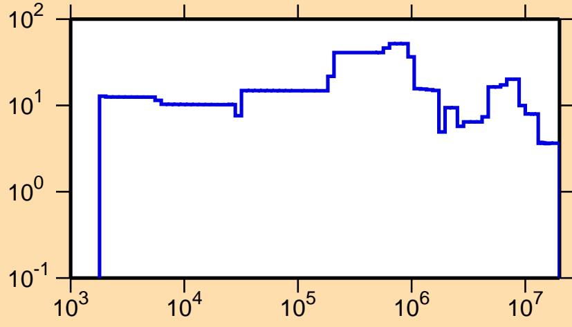
\Delta\sigma/\sigma vs. E for ^{258}\text{Md}(n, el.)
