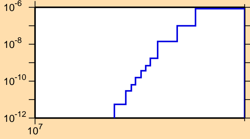
\sigma vs. E for ^{258}\text{Md}(n,2np)
