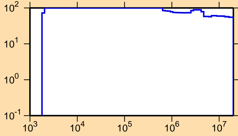
\Delta\sigma/\sigma vs. E for ^{258}\text{Md}(n,n\text{cont.})
