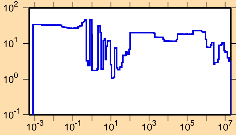
\Delta\sigma/\sigma vs. E for ^{258}\text{Md}(n,\text{tot.})
