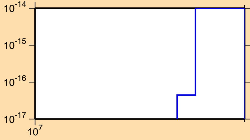
\sigma vs. E for ^{258}\text{Md} (mt 34)
