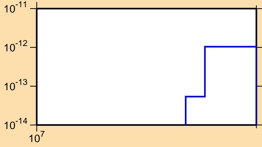
\sigma vs. E for ^{258}\text{Md}(n,3n\alpha)
