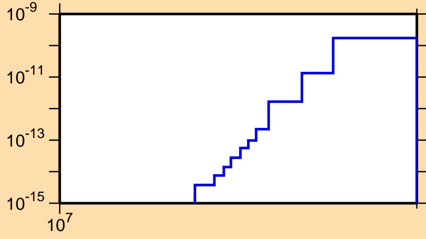
\sigma vs. E for ^{258}\text{Md}(n,\text{He3})
