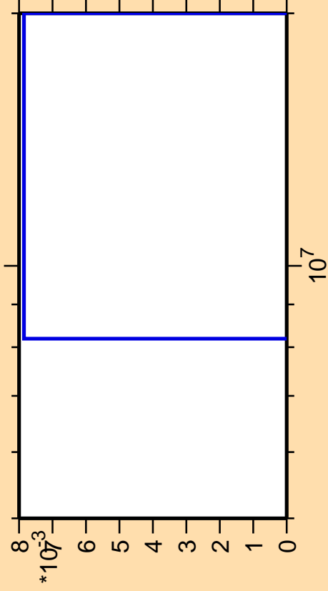
\Delta\sigma/\sigma vs. E for ^{258}\text{Md}(n,3n\alpha)
