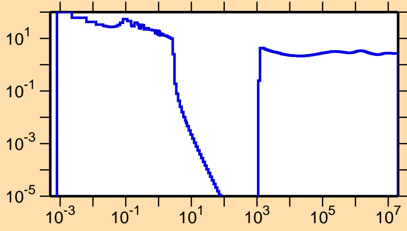
\sigma vs. E for ^{259}\text{Md}(n,f)
