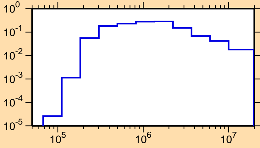
\sigma vs. E for ^{259}\text{Md}(n,n_1)
