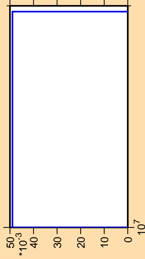
\Delta\sigma/\sigma vs. E for ^{259}\text{Md}(n,\text{He3})
