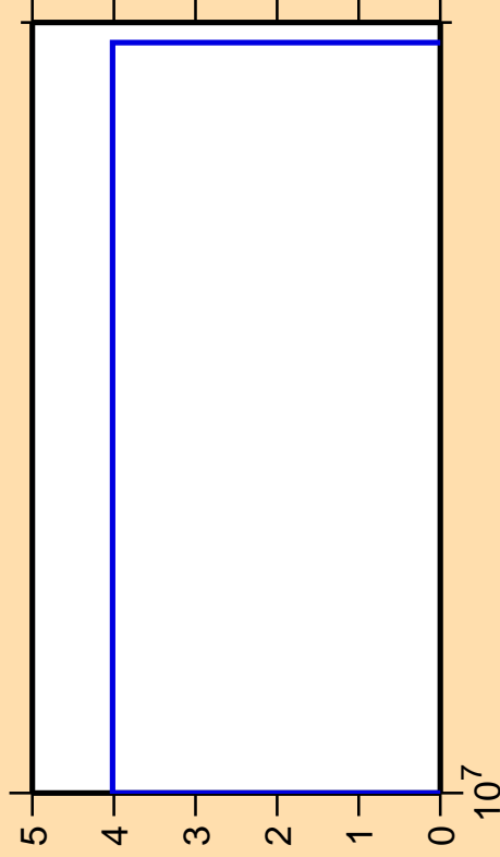
\Delta\sigma/\sigma vs. E for ^{259}\text{Md}(n,2np)
