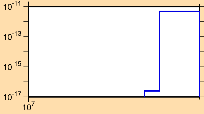
\sigma vs. E for ^{260}\text{Md}(\text{mt } 11)
