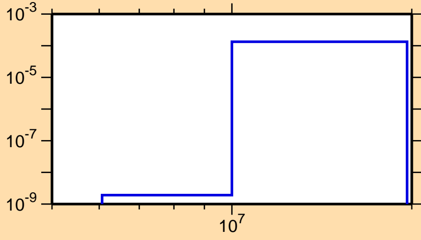
\sigma vs. E for ^{260}\text{Md}(n,t)
