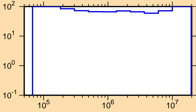
\Delta\sigma/\sigma vs. E for ^{260}\text{Md}(n,n\text{cont.})
