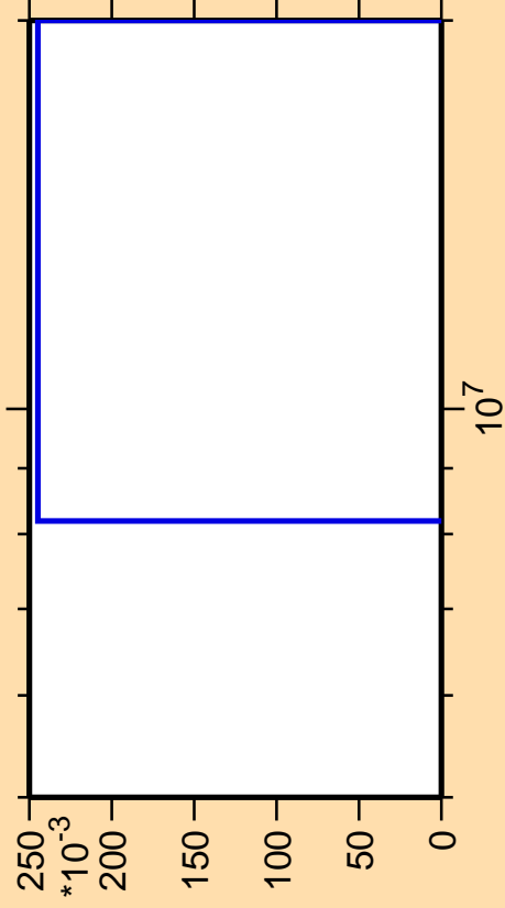
\Delta\sigma/\sigma vs. E for ^{260}\text{Md}(n,3n\alpha)
