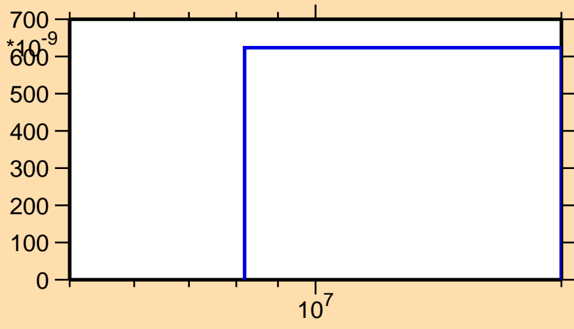
\sigma vs. E for ^{260}\text{Md}(n,nd)
