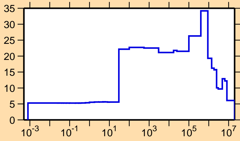
\Delta\sigma/\sigma vs. E for ^{260}\text{Md}(n,el.)
