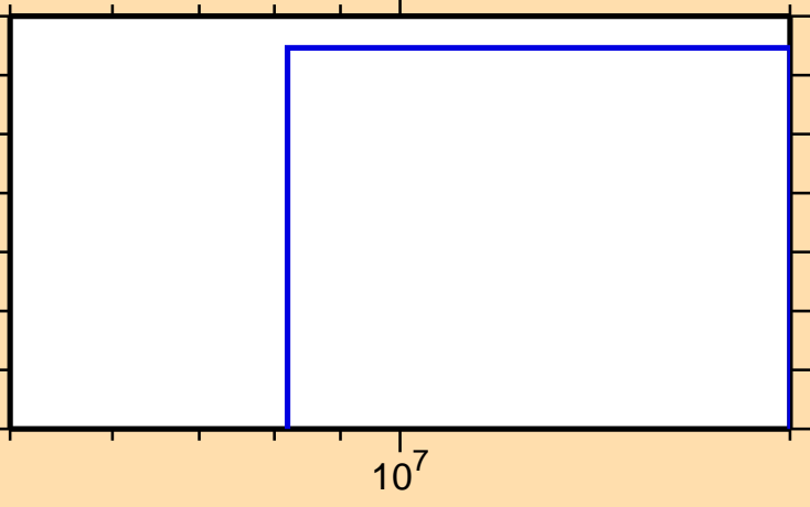
\sigma vs. E for ^{260}\text{Md}(n,nt)
