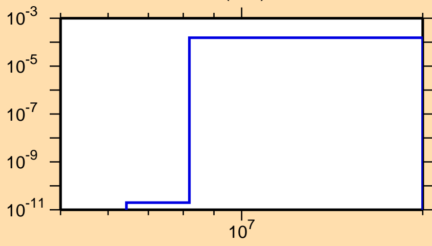
\sigma vs. E for ^{260}\text{Md}(n,d)
