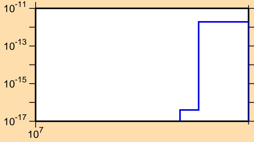
\sigma vs. E for ^{261}\text{Md} (mt 11)
