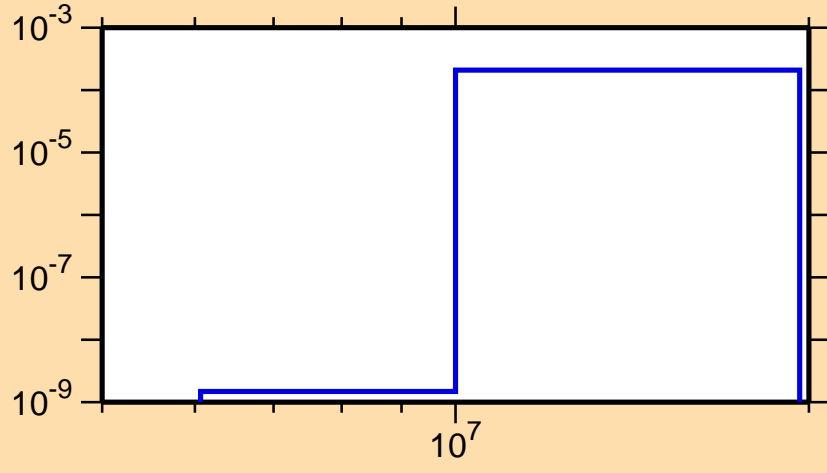
\sigma vs. E for ^{261}\text{Md}(n,d)
