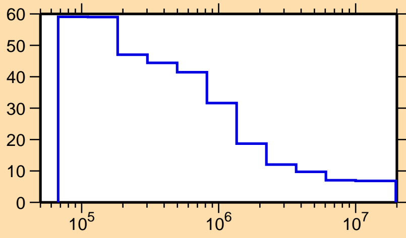
\Delta\sigma/\sigma vs. E for ^{261}\text{Md}(n,n\text{onel.})
