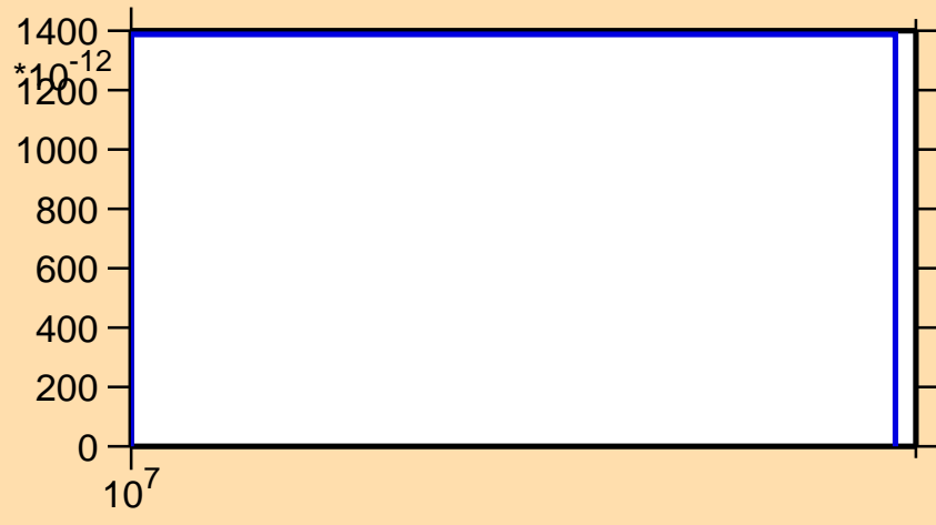
\sigma vs. E for ^{261}\text{Md}(n,2np)
