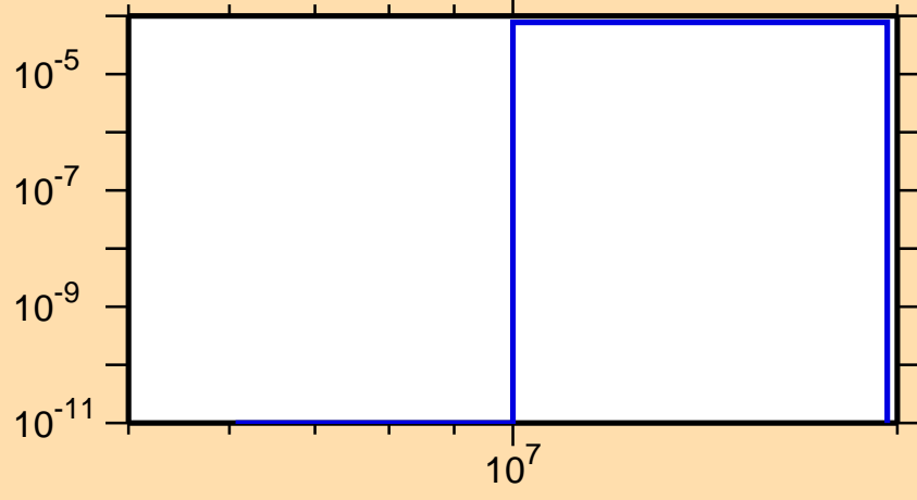
\sigma vs. E for ^{261}\text{Md}(n,np)
