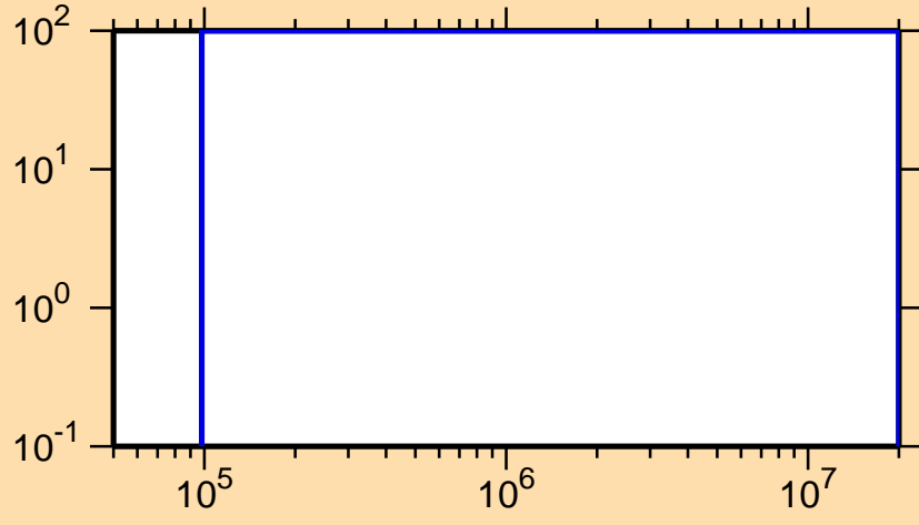
\Delta\sigma/\sigma vs. E for ^{262}\text{Md}(n,n\text{cont.})
