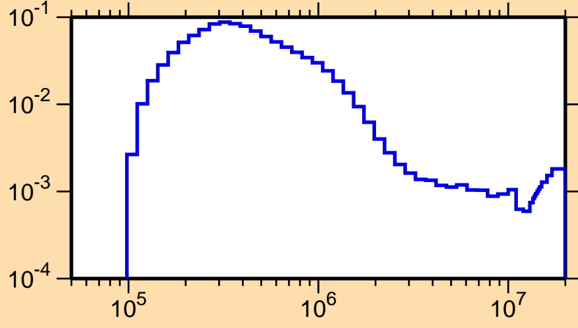
\sigma vs. E for ^{262}\text{Md}(n,n\text{cont.})
