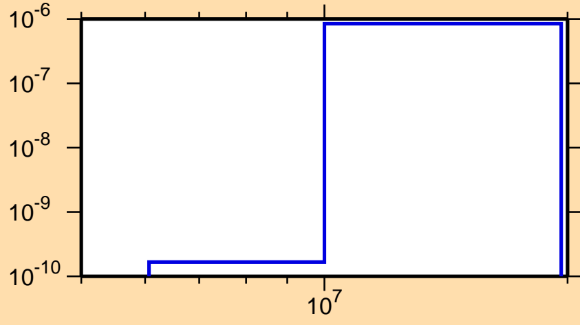
\sigma vs. E for ^{262}\text{Md}(n,t)
