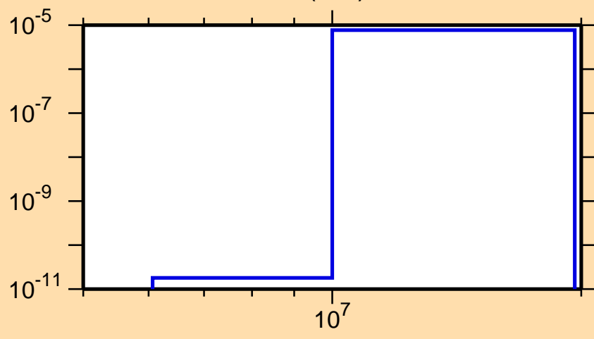
\sigma vs. E for ^{262}\text{Md}(n,d)
