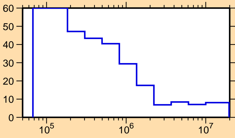
\Delta\sigma/\sigma vs. E for ^{262}\text{Md}(n,\text{nonel.})
