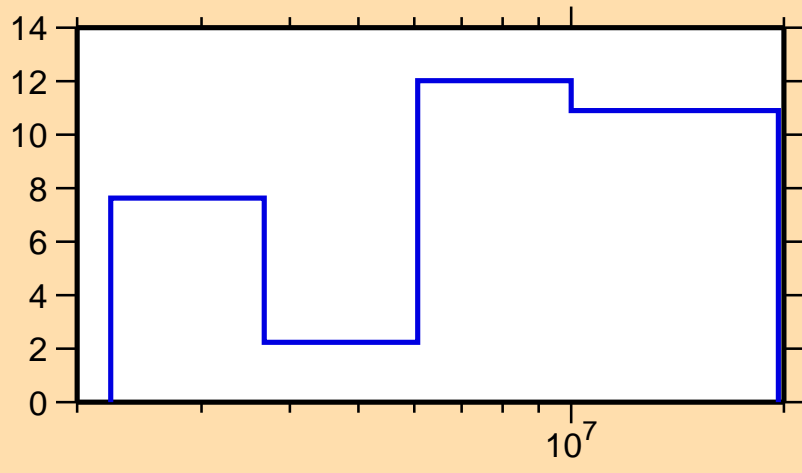
\Delta\sigma/\sigma vs. E for ^{262}\text{Md}(n,\text{el.})
