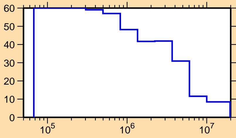
\Delta\sigma/\sigma vs. E for ^{262}\text{Md}(n,f)
