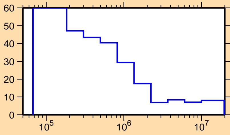
\Delta\sigma/\sigma vs. E for ^{262}\text{Md}(n,n\text{onel.})
