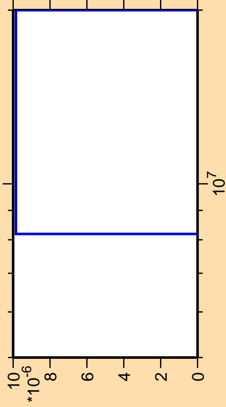
\Delta\sigma/\sigma vs. E for ^{262}\text{Md}(n,\text{He3})
