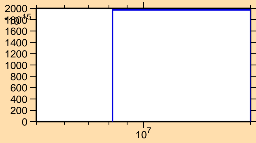
\sigma vs. E for ^{262}\text{Md}(n,2n\alpha)
