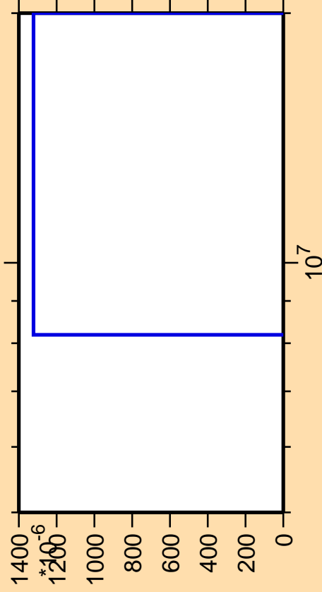
\Delta\sigma/\sigma vs. E for ^{262}\text{Md}(n,3n\alpha)
