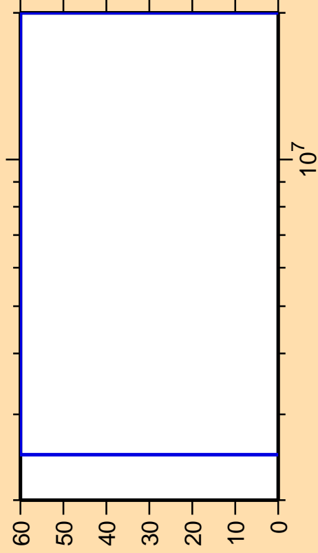
\Delta\sigma/\sigma vs. E for ^{262}\text{Md}(n,\alpha)
