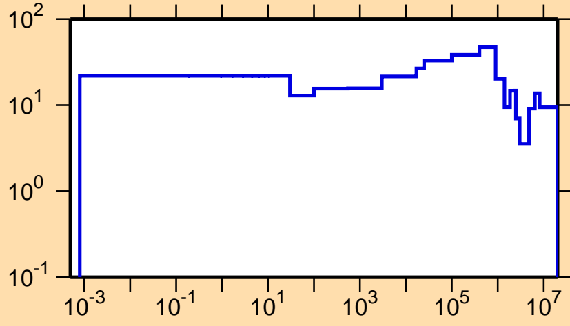
\Delta\sigma/\sigma vs. E for ^{262}\text{Md}(n,el.)
