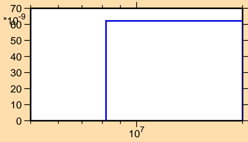
\sigma vs. E for ^{262}\text{Md}(n,nd)
