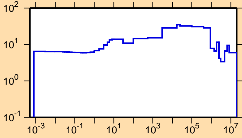
\Delta\sigma/\sigma vs. E for ^{262}\text{Md}(n,\text{tot.})
