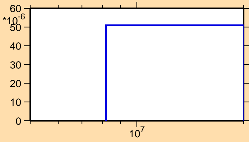
\sigma vs. E for ^{262}\text{Md}(n,3n)
