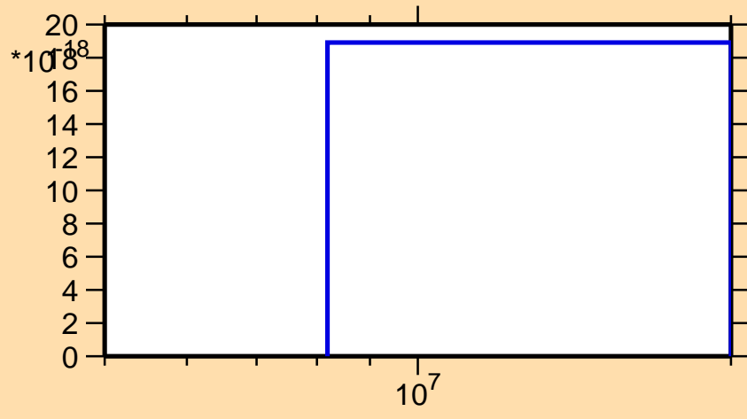
\sigma vs. E for ^{262}\text{Md}(n,\text{He3})
