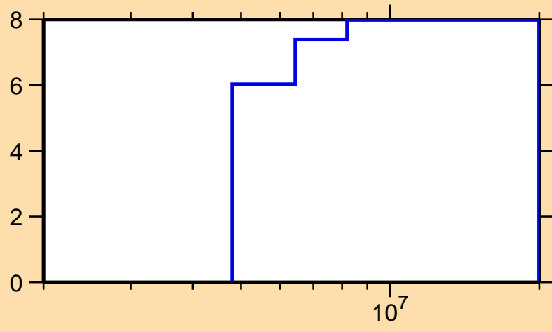
\Delta\sigma/\sigma vs. E for ^{262}\text{Md}(n,\text{nonel.})
