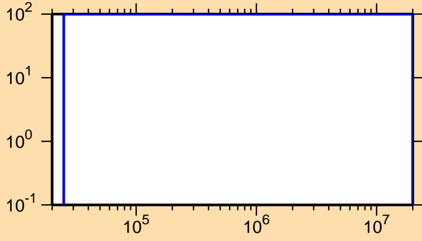
\Delta\sigma/\sigma vs. E for ^{262}\text{Md}(n,n_1)
