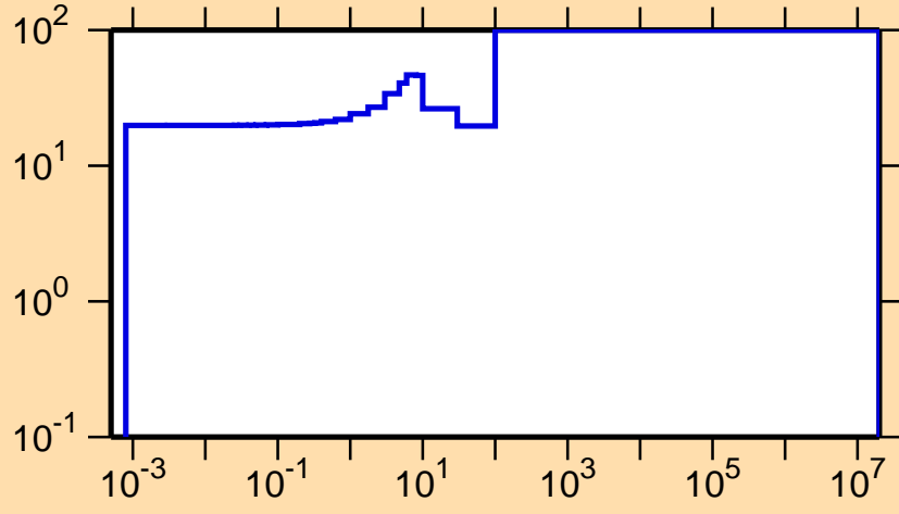
\Delta\sigma/\sigma vs. E for ^{262}\text{Md}(n,\gamma)
