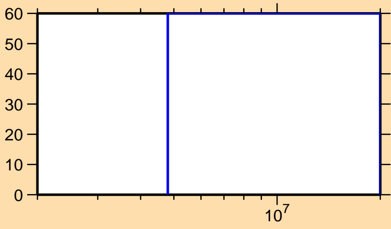
\Delta\sigma/\sigma vs. E for ^{262}\text{Md}(n,2n)
