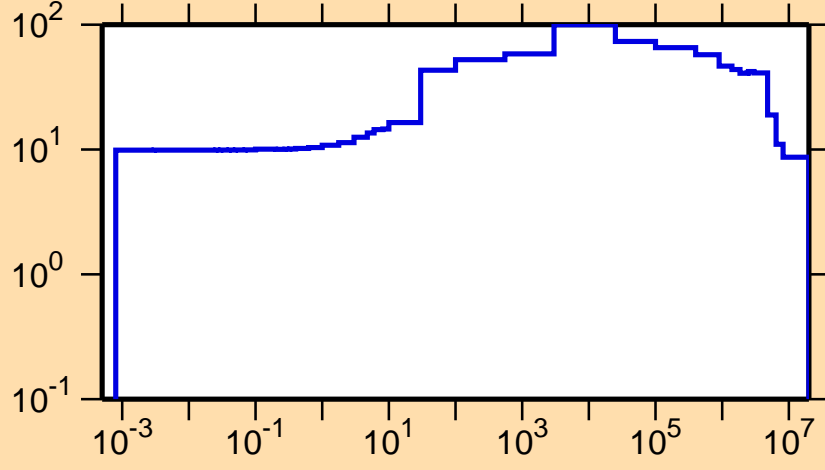
\Delta\sigma/\sigma vs. E for ^{262}\text{Md}(n,f)
