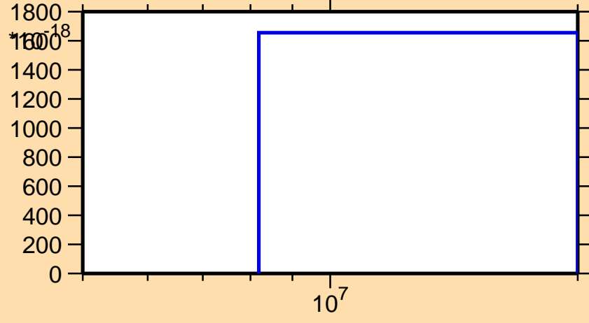
\sigma vs. E for ^{262}\text{Md}(n,3n\alpha)
