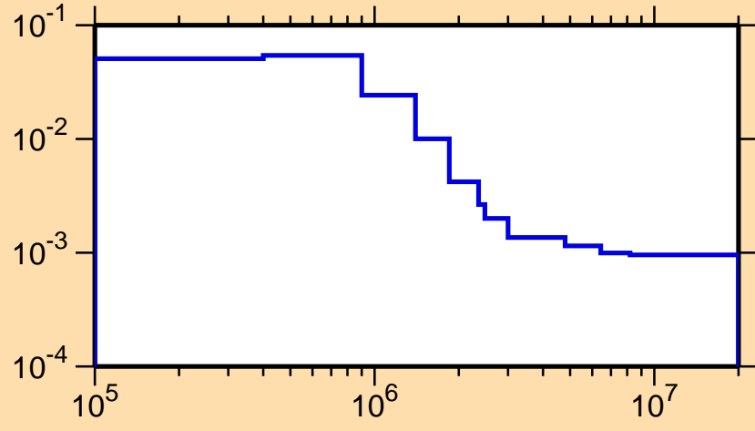
\sigma vs. E for ^{262}\text{Md}(n,\text{inel.})
