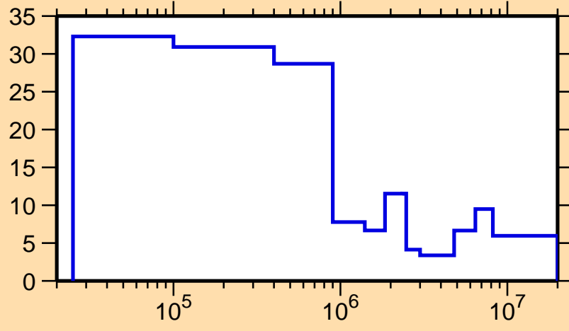
\Delta\sigma/\sigma vs. E for ^{262}\text{Md}(n,\text{tot.})
