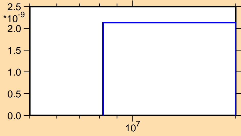
\sigma vs. E for ^{262}\text{Md}(n,np)
