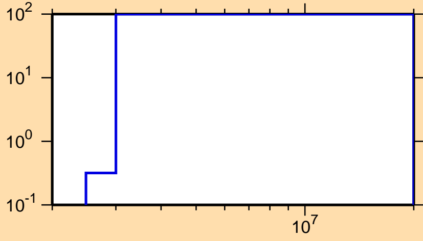
\Delta\sigma/\sigma vs. E for ^{262}\text{Md}(n,p)
