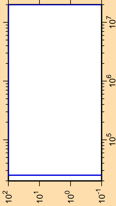
\Delta\sigma/\sigma vs. E for ^{262}\text{Md}(n,\text{inel.})
