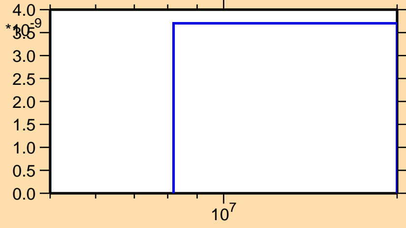
\sigma vs. E for ^{262}\text{Md}(n,2np)
