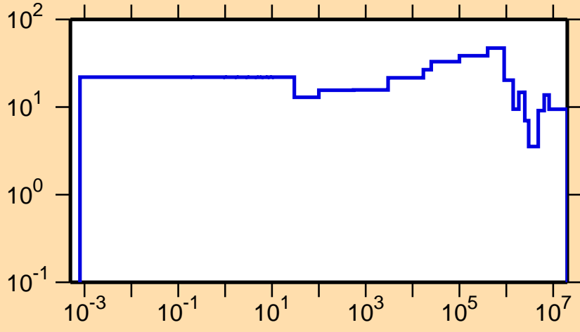
\Delta\sigma/\sigma vs. E for ^{262}\text{Md}(n,\text{el.})
