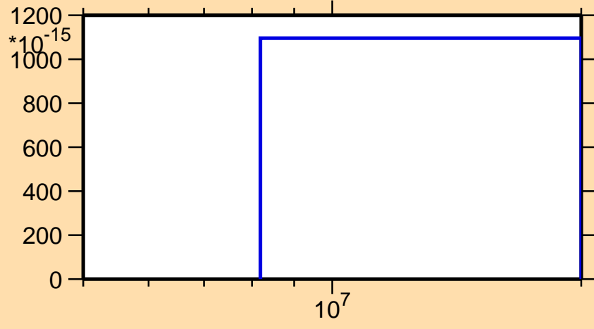
\sigma vs. E for ^{262}\text{Md}(n,nt)
