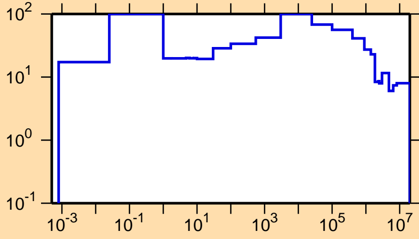
\Delta\sigma/\sigma vs. E for ^{262}\text{Md}(n,\text{nonel.})
