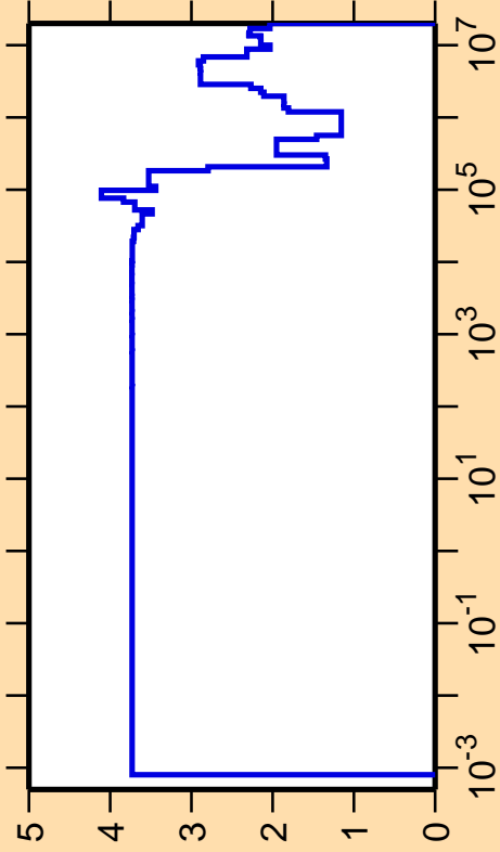
\Delta\sigma/\sigma vs. E for ^{24}\text{Mg}(n,\text{el.})
