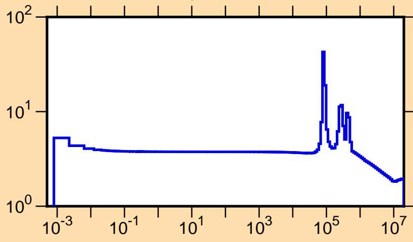
\sigma vs. E for ^{24}\text{Mg}(n,\text{tot.})
