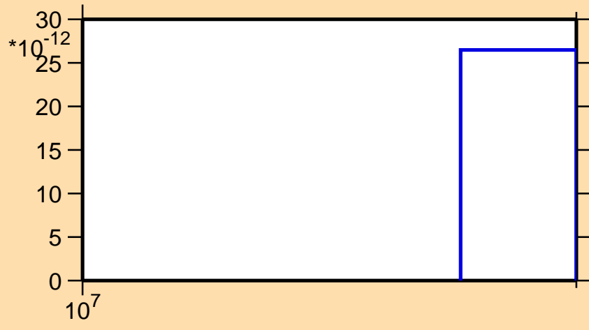
\sigma vs. E for ^{24}\text{Mg}(n,\text{pd})
