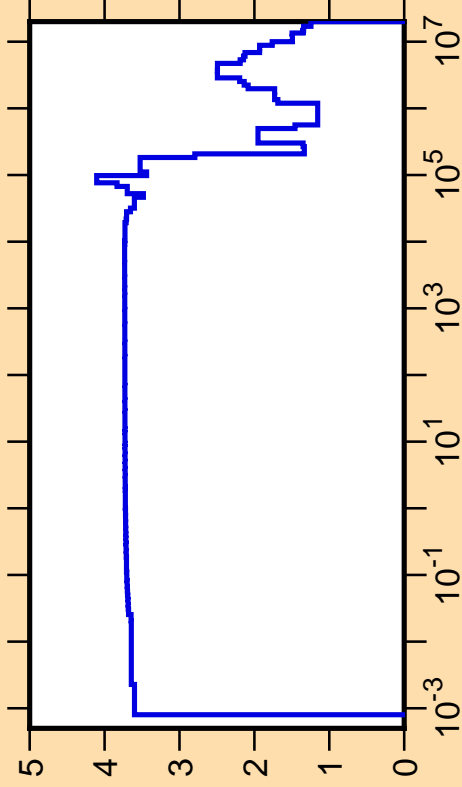
\Delta\sigma/\sigma vs. E for ^{24}\text{Mg}(n,\text{tot.})
