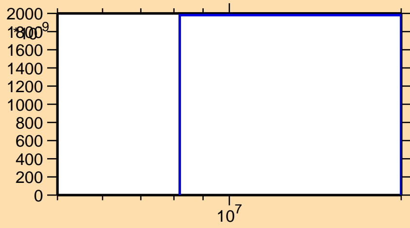
\sigma vs. E for ^{24}\text{Mg}(n,\text{He}3)
