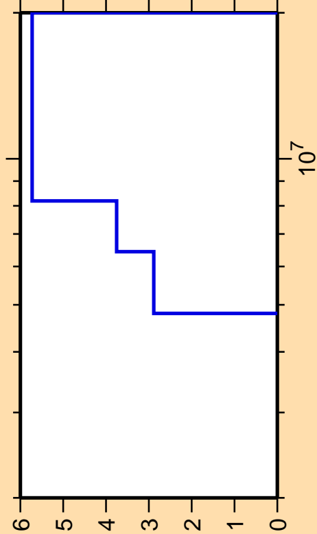
\Delta\sigma/\sigma vs. E for ^{24}\text{Mg}(n,n_4)
