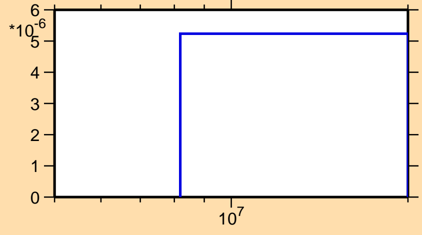
\sigma vs. E for ^{24}\text{Mg}(n,2n)
