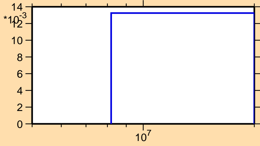
\sigma vs. E for ^{24}\text{Mg}(n,d)
