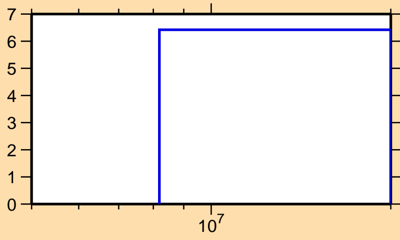
\Delta\sigma/\sigma vs. E for ^{24}\text{Mg}(n,n\text{cont.})
