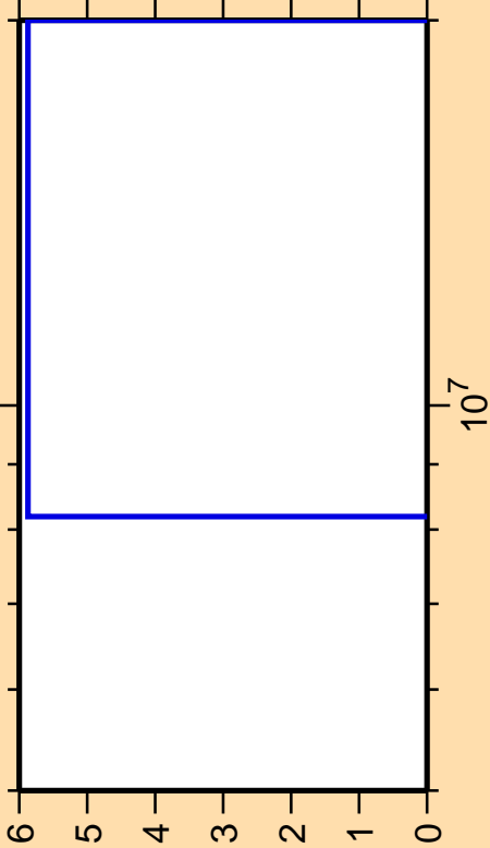
\Delta\sigma/\sigma vs. E for ^{24}\text{Mg}(n,n_1)
