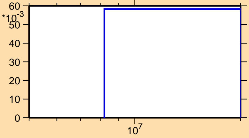
\sigma vs. E for ^{24}\text{Mg}(n,np)
