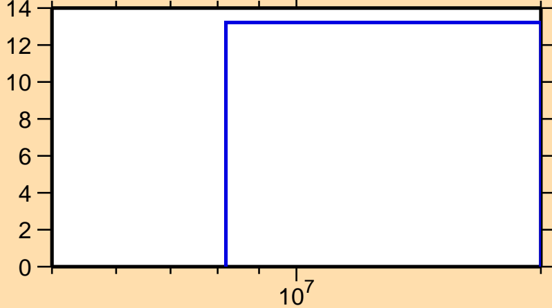
\Delta\sigma/\sigma vs. E for ^{24}\text{Mg}(n,2n)
