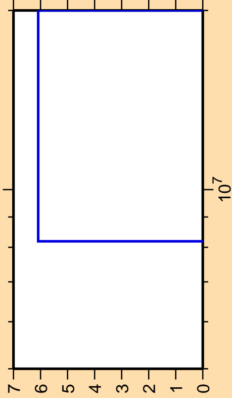
\Delta\sigma/\sigma vs. E for ^{24}\text{Mg}(n,n\alpha)
