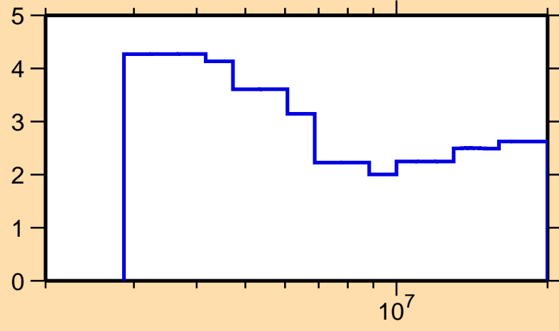
\Delta\sigma/\sigma vs. E for ^{25}\text{Mg}(n,el.)
