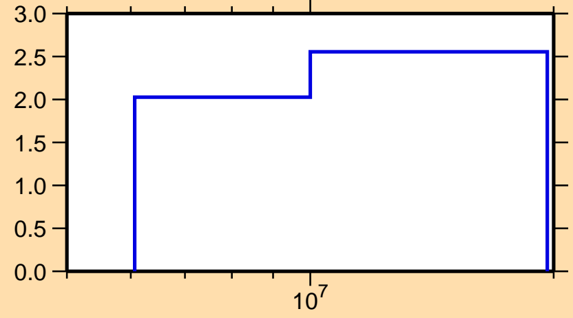
\Delta\sigma/\sigma vs. E for ^{25}\text{Mg}(n,\text{nonel.})
