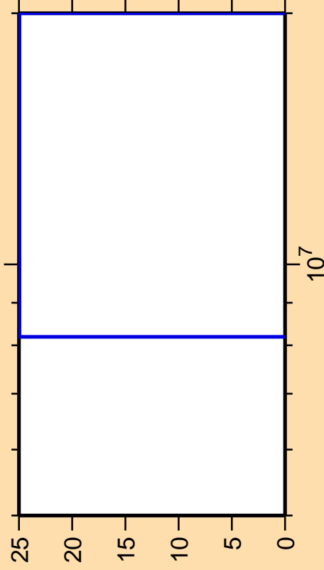
\Delta\sigma/\sigma vs. E for ^{25}\text{Mg}(n,nd)
