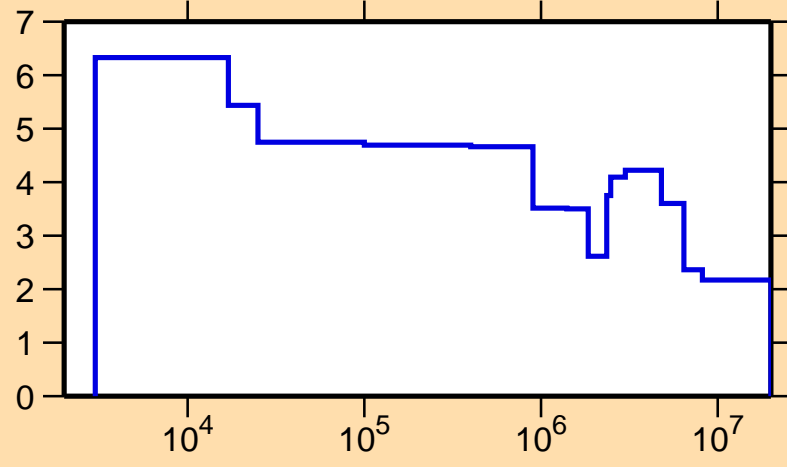
\Delta\sigma/\sigma vs. E for ^{25}\text{Mg}(n,\text{el.})
