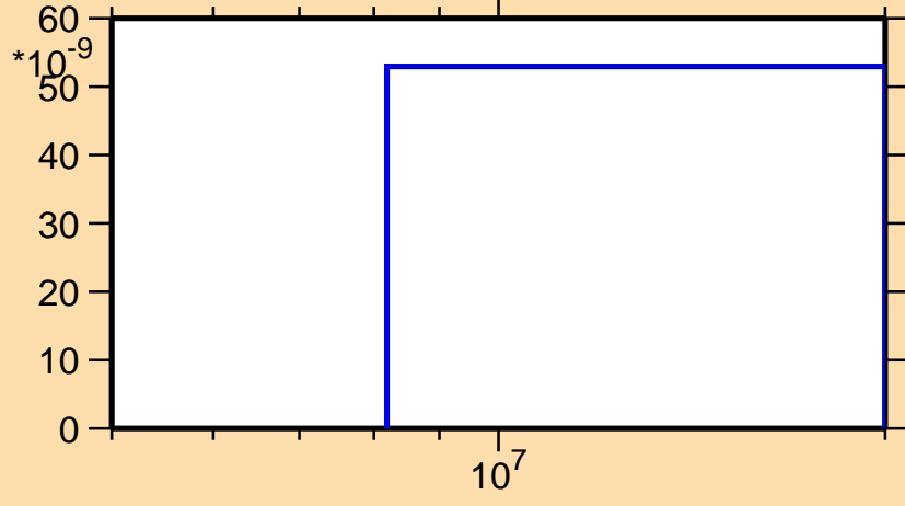
\sigma vs. E for ^{25}\text{Mg}(n,nd)
