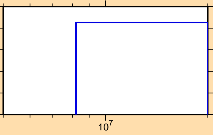
\sigma vs. E for ^{25}\text{Mg}(n,\text{He}3)
