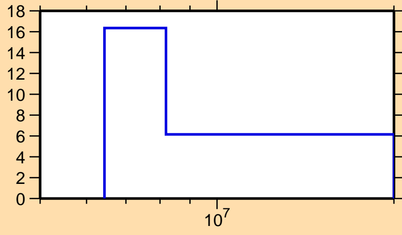
\Delta\sigma/\sigma vs. E for ^{25}\text{Mg}(n,2n)
