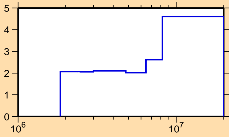
\Delta\sigma/\sigma vs. E for ^{25}\text{Mg}(n,\text{inel.})
