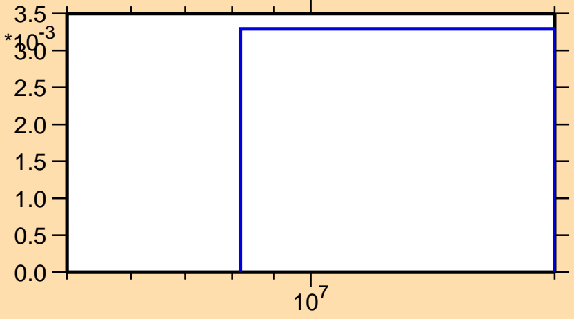
\sigma vs. E for ^{25}\text{Mg}(n,np)
