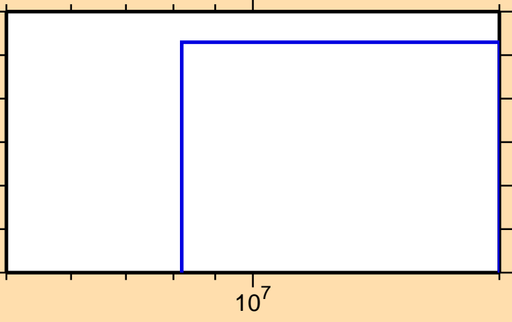
\sigma vs. E for ^{25}\text{Mg}(n,nd)
