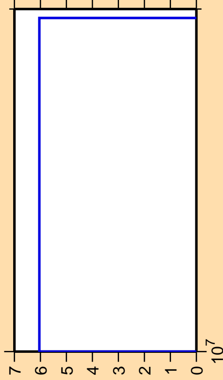
\Delta\sigma/\sigma vs. E for ^{26}\text{Mg}(n,2n)
