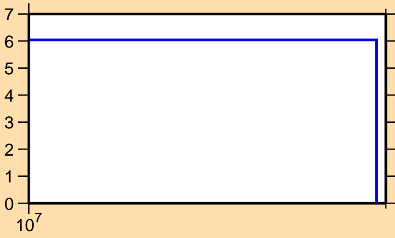
\Delta\sigma/\sigma vs. E for ^{26}\text{Mg}(n,2n)
