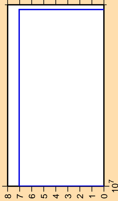
\Delta\sigma/\sigma vs. E for ^{26}\text{Mg}(n,n\text{cont.})
