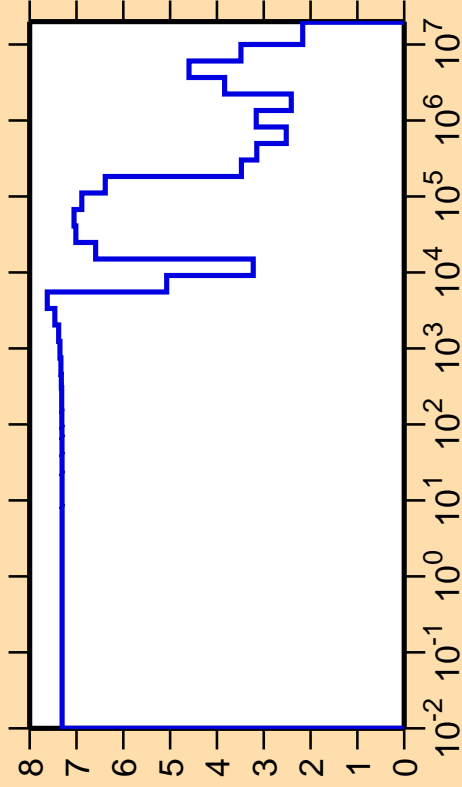
\Delta\sigma/\sigma vs. E for ^{26}\text{Mg}(n,\text{el.})
