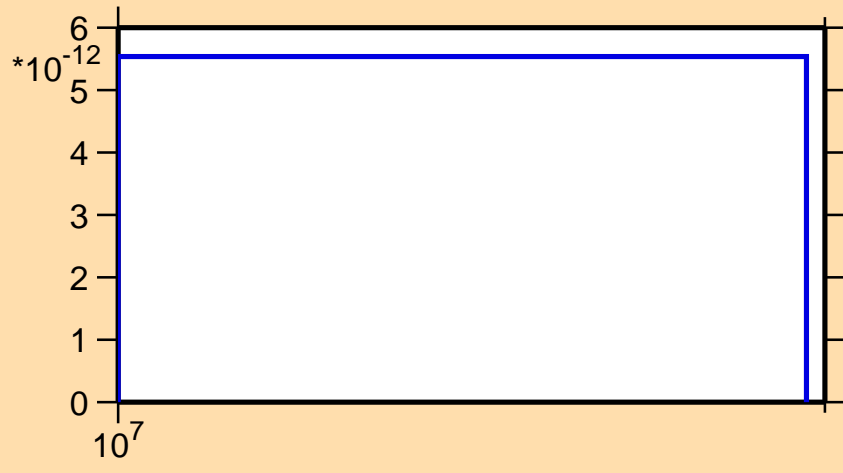
\sigma vs. E for ^{26}\text{Mg}(n,\text{He}3)
