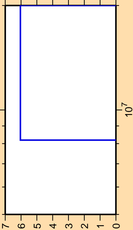
\Delta\sigma/\sigma vs. E for ^{26}\text{Mg}(n,2n)
