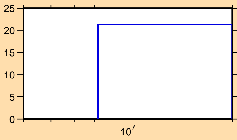
\Delta\sigma/\sigma vs. E for ^{26}\text{Mg}(n,p)
