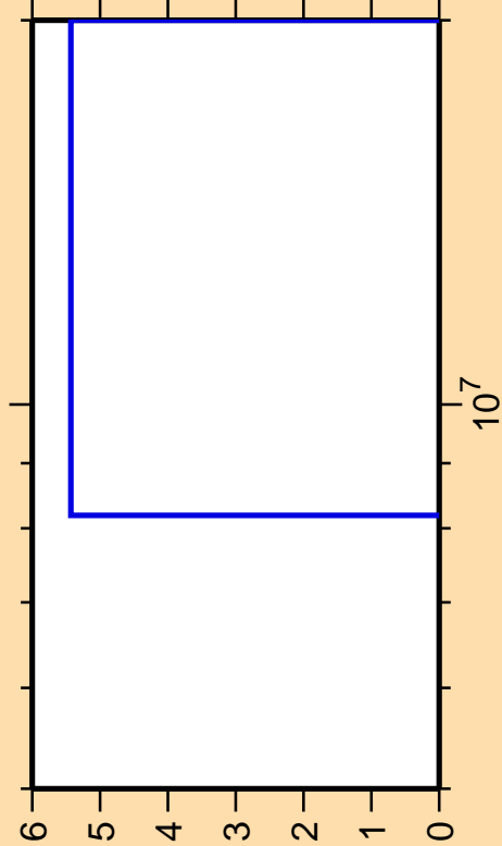
\Delta\sigma/\sigma vs. E for ^{26}\text{Mg}(n,\text{He}3)
