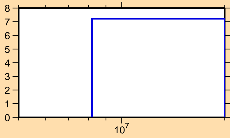
\Delta\sigma/\sigma vs. E for ^{26}\text{Mg}(n,n\text{cont.})
