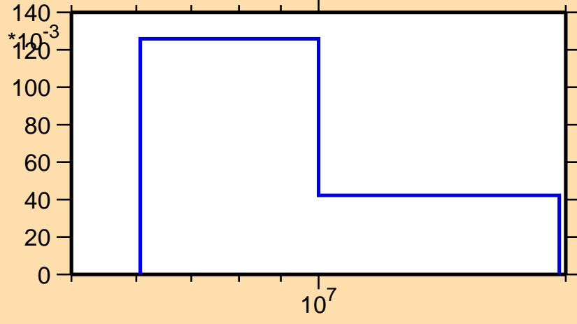
\sigma vs. E for ^{27}\text{Mg}(n,n\text{cont.})
