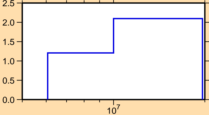
\Delta\sigma/\sigma vs. E for ^{27}\text{Mg}(n,\text{nonel.})
