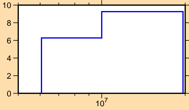
\Delta\sigma/\sigma vs. E for ^{27}\text{Mg}(n,\text{inel.})
