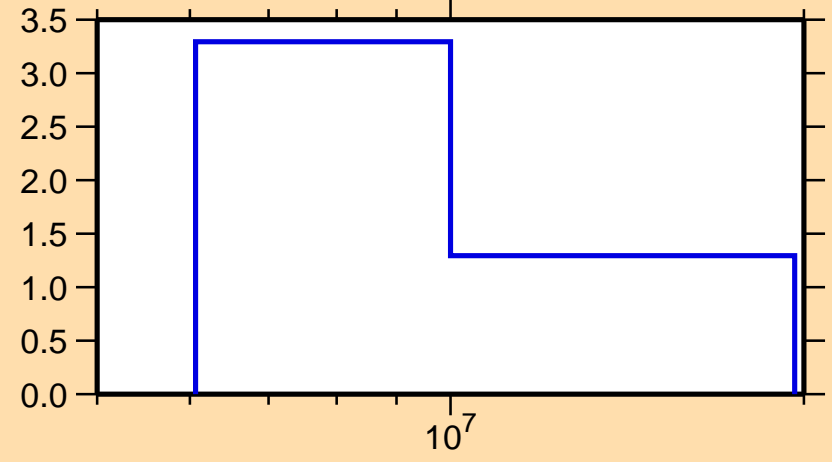
\Delta\sigma/\sigma vs. E for ^{27}\text{Mg}(n,\text{el.})
