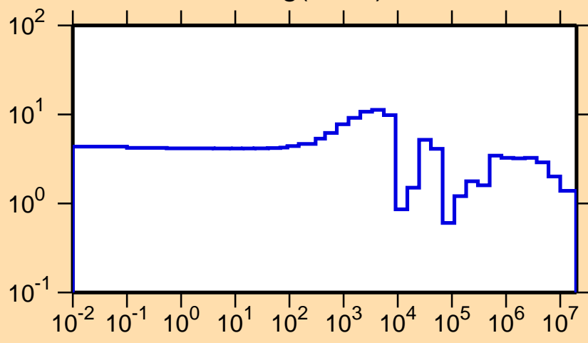
\Delta\sigma/\sigma vs. E for ^{27}\text{Mg}(n,\text{tot.})
