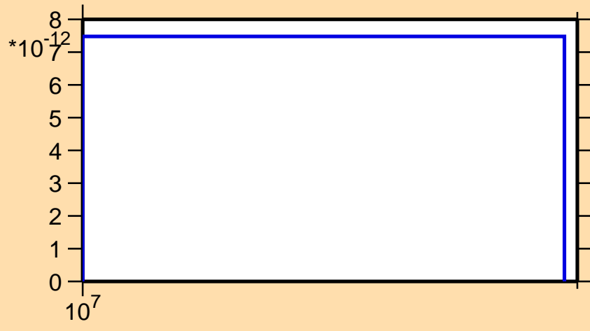
\sigma vs. E for ^{27}\text{Mg}(n,2n\alpha)
