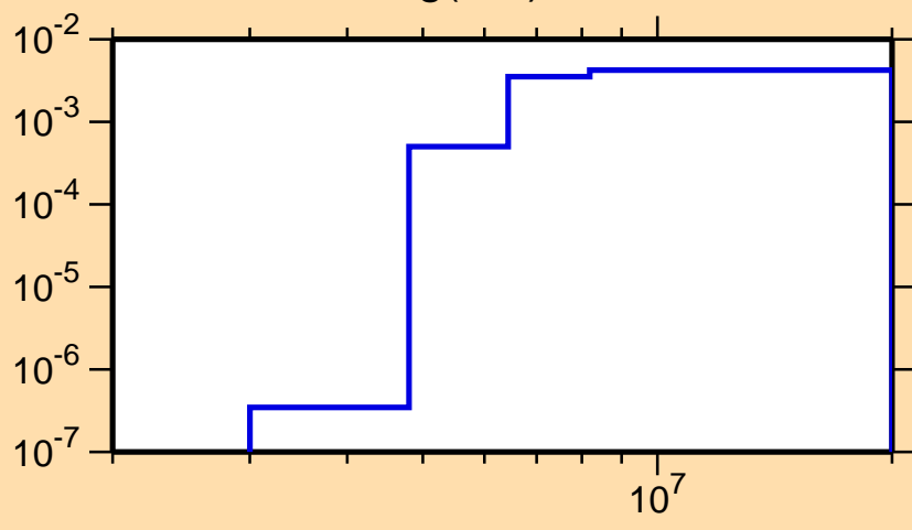
\sigma vs. E for ^{27}\text{Mg}(n,\alpha)
