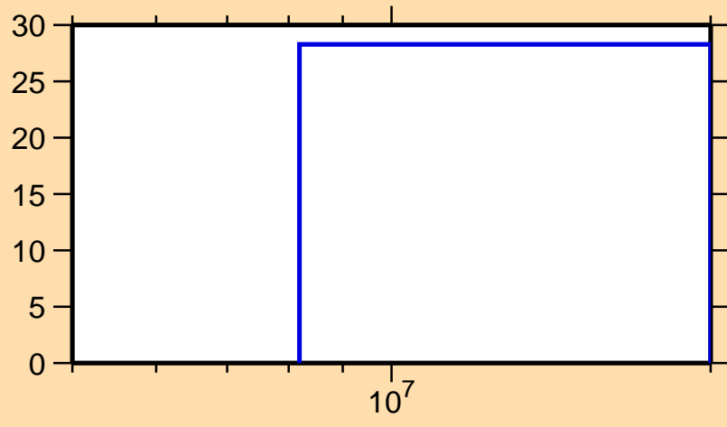
\Delta\sigma/\sigma vs. E for ^{27}\text{Mg}(n,n_1)
