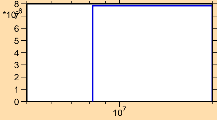
\sigma vs. E for ^{27}\text{Mg}(n,np)
