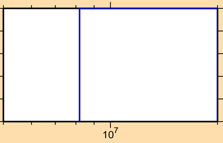
\sigma vs. E for ^{27}\text{Mg}(n,d)
