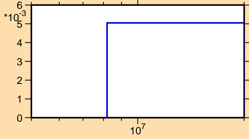
\sigma vs. E for ^{27}\text{Mg}(n,p)
