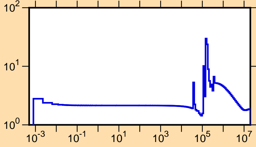
\sigma vs. E for ^{28}\text{Mg}(n,\text{tot.})
