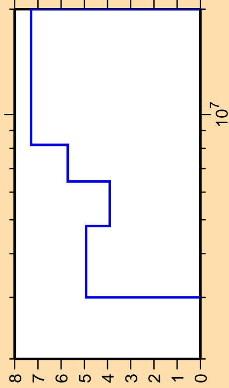
\Delta\sigma/\sigma vs. E for ^{28}\text{Mg}(n,n_4)
