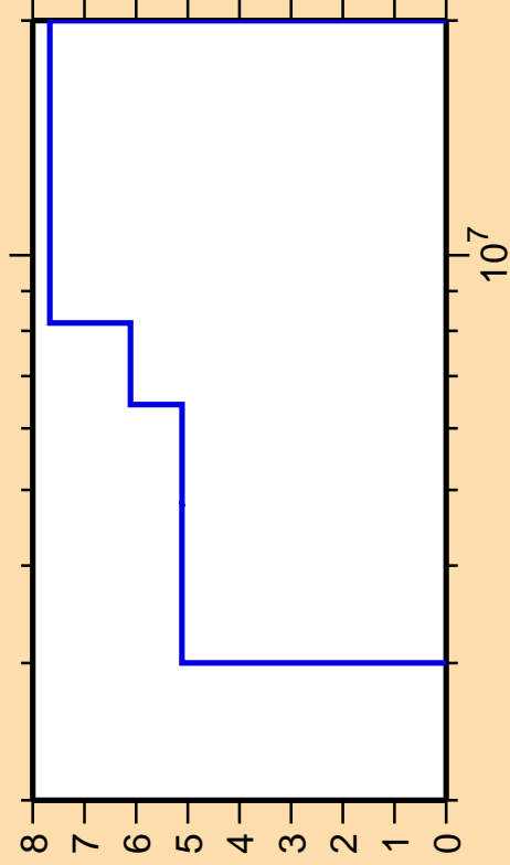
\Delta\sigma/\sigma vs. E for ^{28}\text{Mg}(n,n_2)
