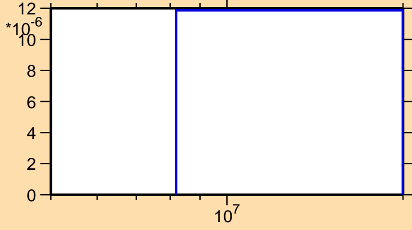
\sigma vs. E for ^{28}\text{Mg}(n,p)
