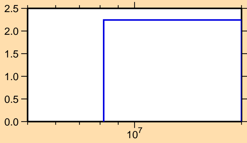
\Delta\sigma/\sigma vs. E for ^{28}\text{Mg}(n,n\text{onel.})
