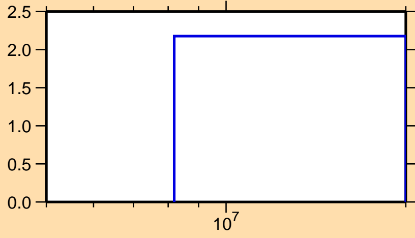
\Delta\sigma/\sigma vs. E for ^{28}\text{Mg}(n,el.)
