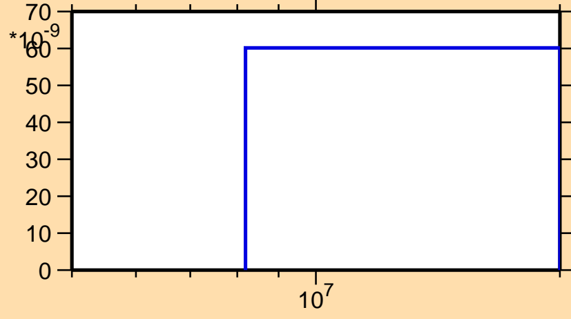
\sigma vs. E for ^{28}\text{Mg}(n,np)
