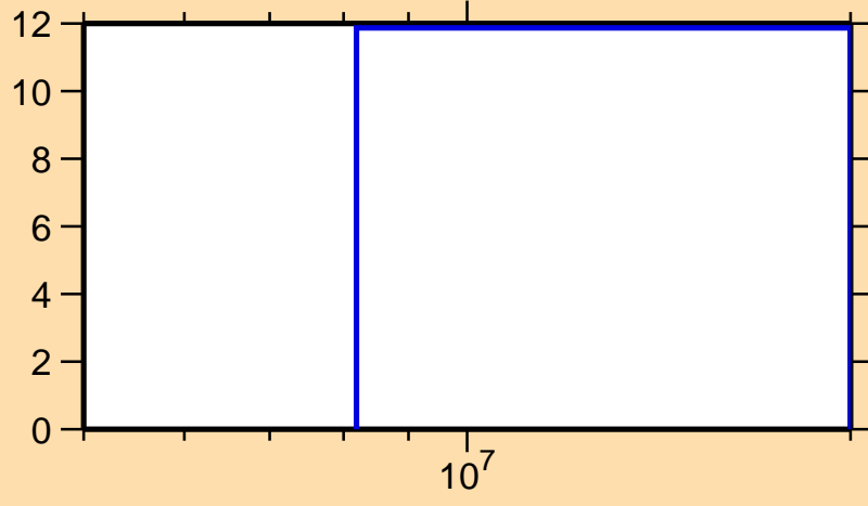
\Delta\sigma/\sigma vs. E for ^{28}\text{Mg}(n,n_1)
