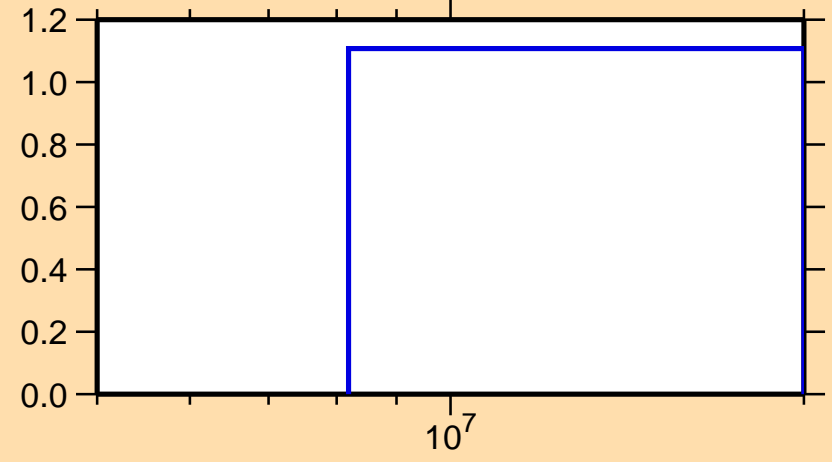
\Delta\sigma/\sigma vs. E for ^{28}\text{Mg}(n,\text{tot.})
