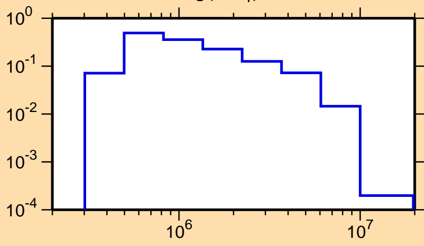
\sigma vs. E for ^{29}\text{Mg}(n,n_1)
