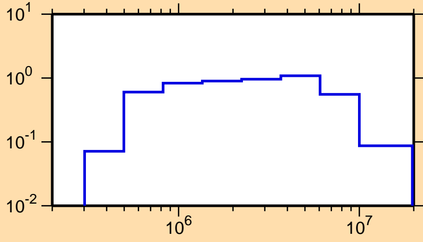
\sigma vs. E for ^{29}\text{Mg}(n,\text{inel.})
