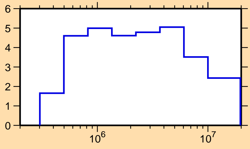
\Delta\sigma/\sigma vs. E for ^{29}\text{Mg}(n,\text{el.})
