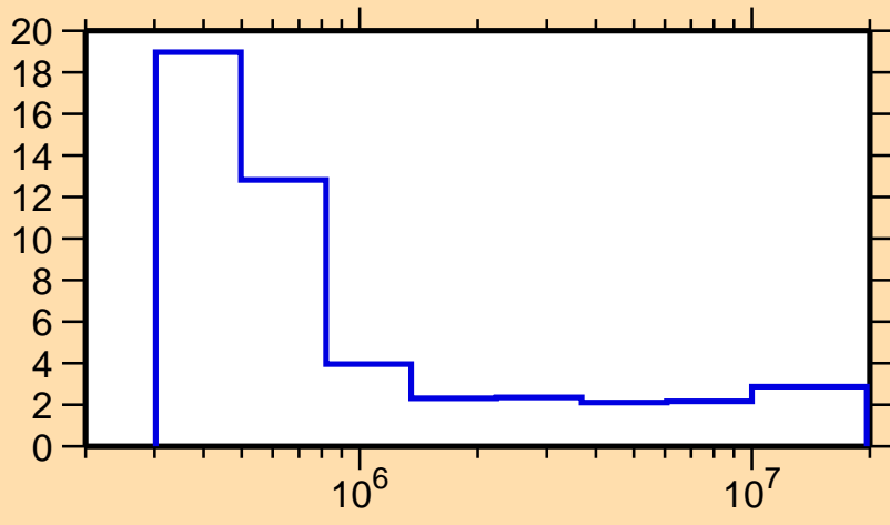
\Delta\sigma/\sigma vs. E for ^{29}\text{Mg}(n,\text{nonel.})
