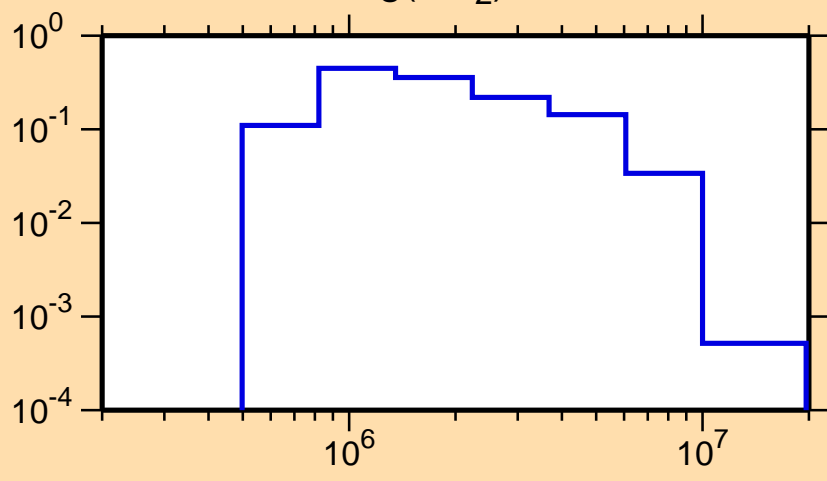
\sigma vs. E for ^{29}\text{Mg}(n,n_2)
