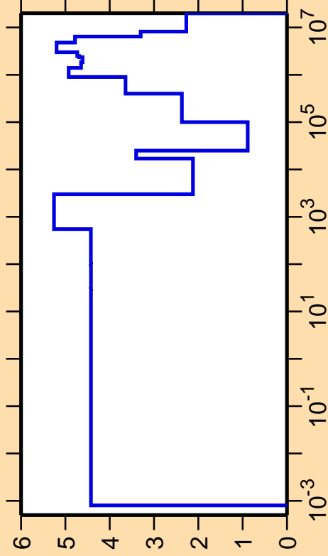
\Delta\sigma/\sigma vs. E for ^{29}\text{Mg}(n,\text{el.})
