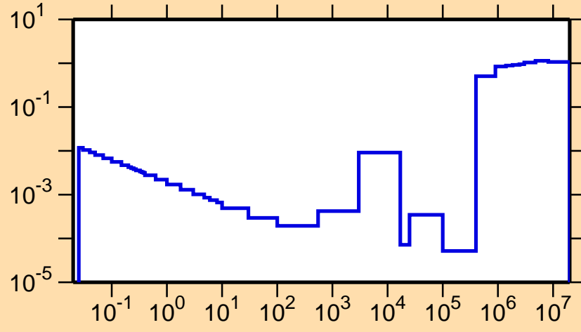
\sigma vs. E for ^{29}\text{Mg}(n,\text{nonel.})
