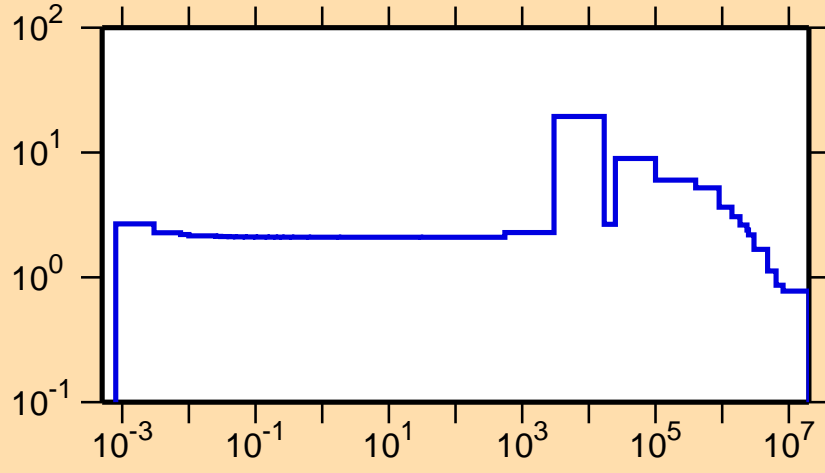
\sigma vs. E for ^{29}\text{Mg}(n,\text{el.})
