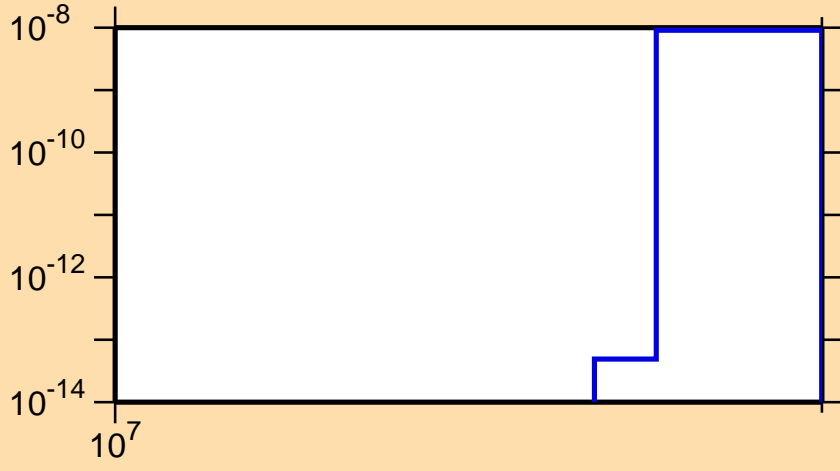
\sigma vs. E for ^{50}\text{Mn} (mt 45)
