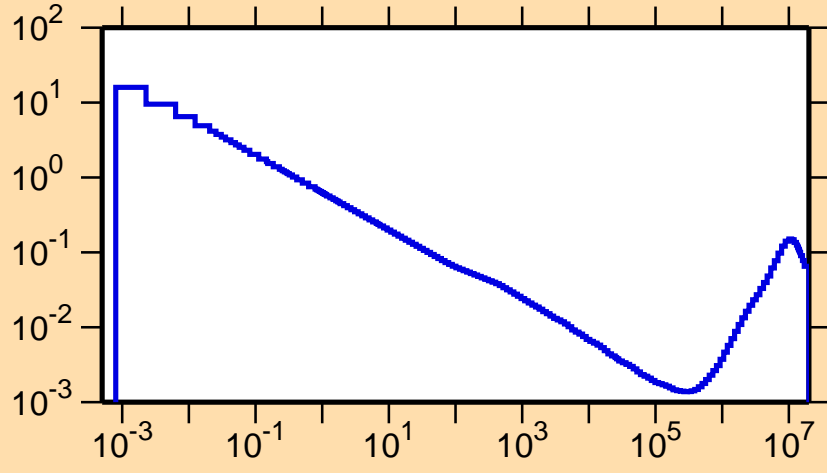
\sigma vs. E for ^{50}\text{Mn}(n,\alpha)
