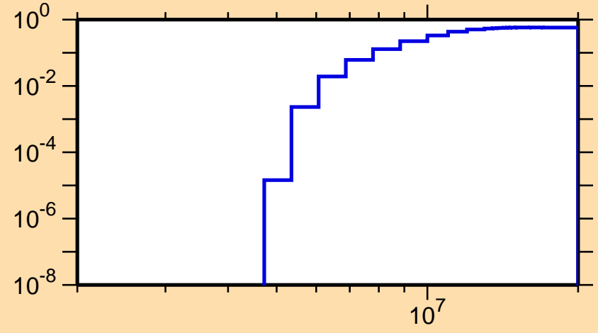
\sigma vs. E for ^{50}\text{Mn}(n,np)
