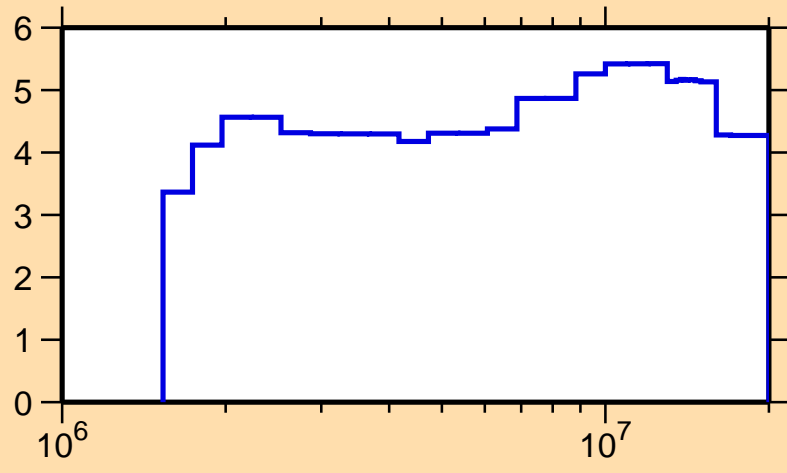
\Delta\sigma/\sigma vs. E for ^{50}\text{Mn}(n,\text{el.})
