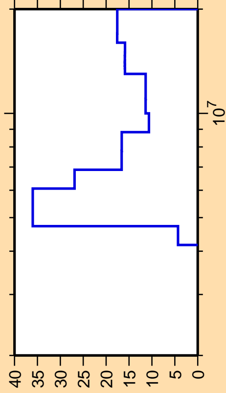
\Delta\sigma/\sigma vs. E for ^{50}\text{Mn}(n,np)
