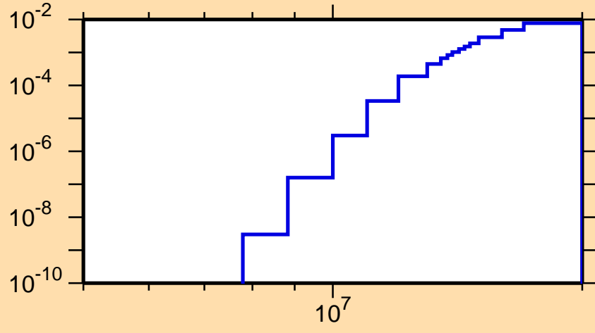
\sigma vs. E for ^{50}\text{Mn}(n,\text{He}3)
