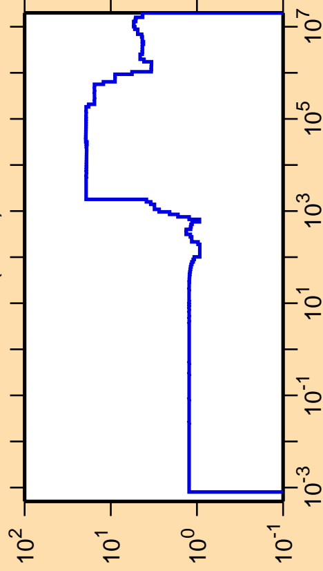
\Delta\sigma/\sigma vs. E for ^{50}\text{Mn}(n,\text{el.})
