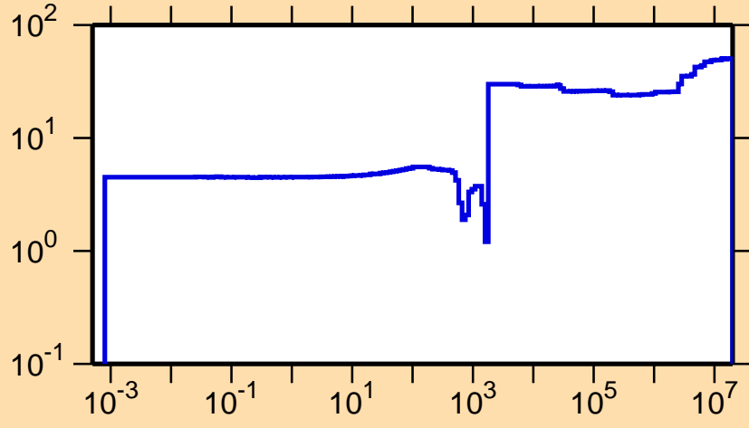
\Delta\sigma/\sigma vs. E for ^{50}\text{Mn}(n,\gamma)
