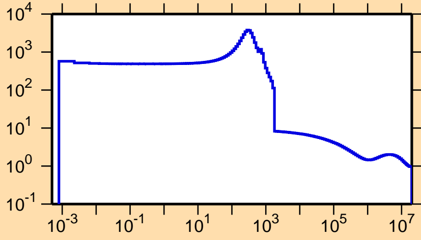
\sigma vs. E for ^{50}\text{Mn}(n,\text{el.})
