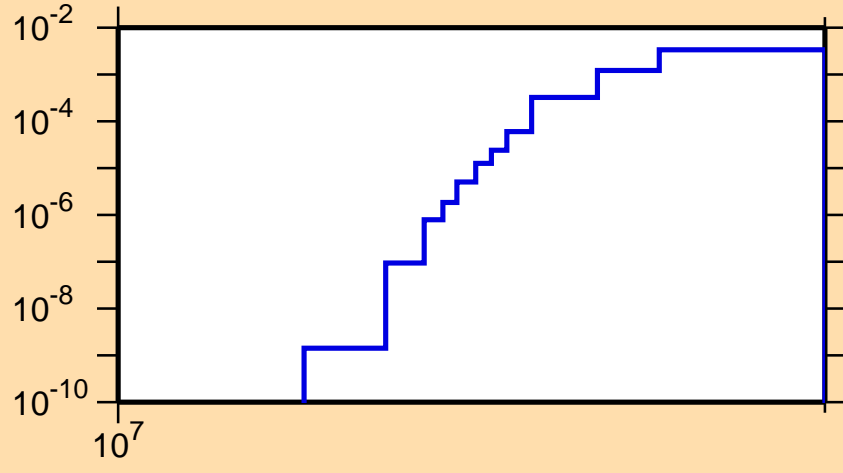
\sigma vs. E for ^{50}\text{Mn}(n,pd)
