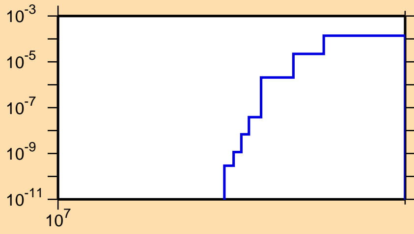
\sigma vs. E for ^{50}\text{Mn}(n,nd)
