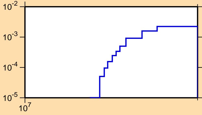
\sigma vs. E for ^{50}\text{Mn}(n,2n)
