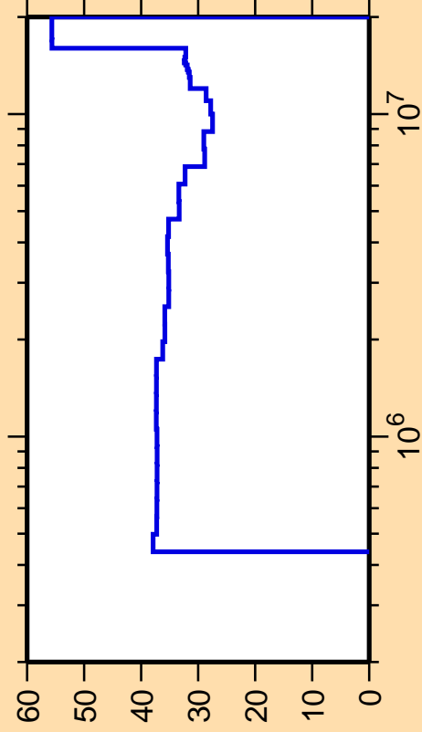
\Delta\sigma/\sigma vs. E for ^{50}\text{Mn}(n,n_3)
