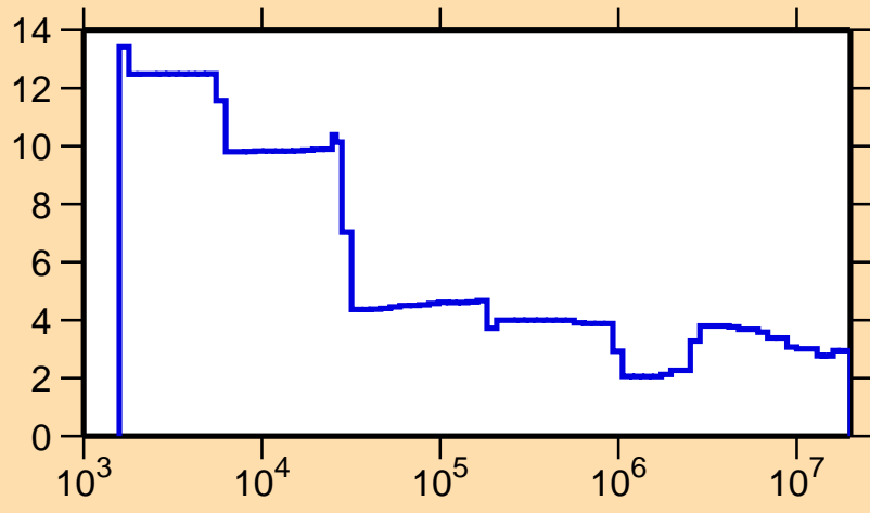
\Delta\sigma/\sigma vs. E for ^{50}\text{Mn}(n,\text{nonel.})
