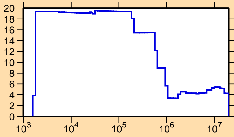
\Delta\sigma/\sigma vs. E for ^{50}\text{Mn}(n,\text{el.})
