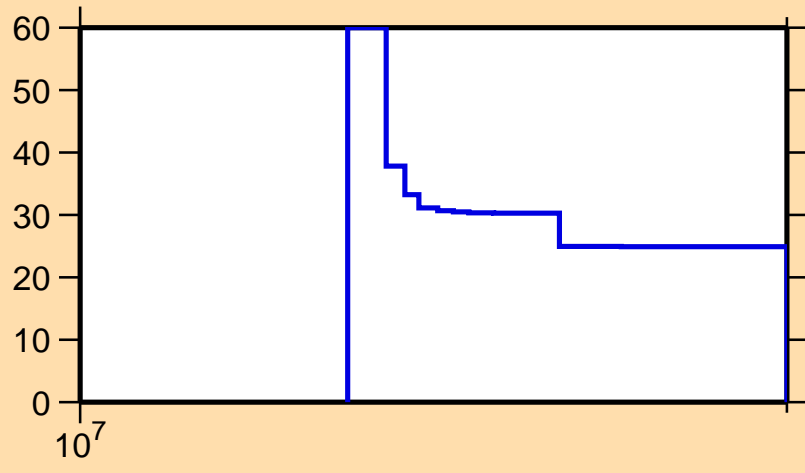
\Delta\sigma/\sigma vs. E for ^{50}\text{Mn}(n,2n)
