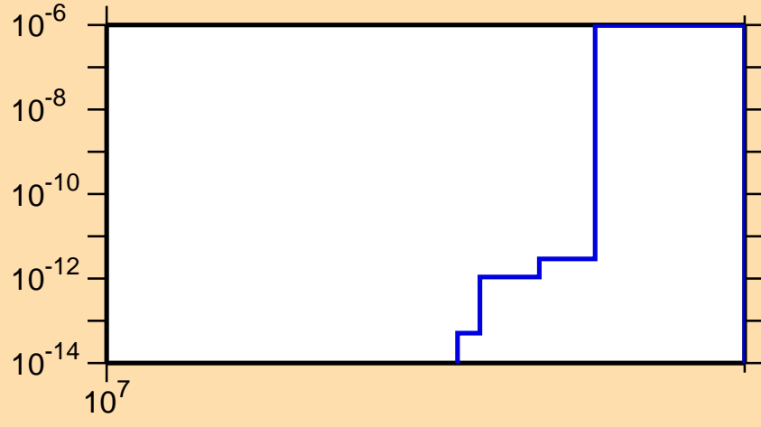
\sigma vs. E for ^{50}\text{Mn}(n,pt)
