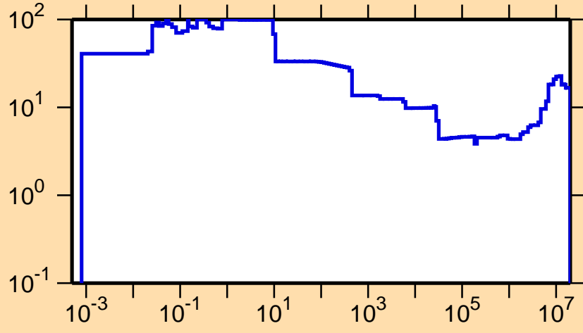
\Delta\sigma/\sigma vs. E for ^{50}\text{Mn}(n,p)
