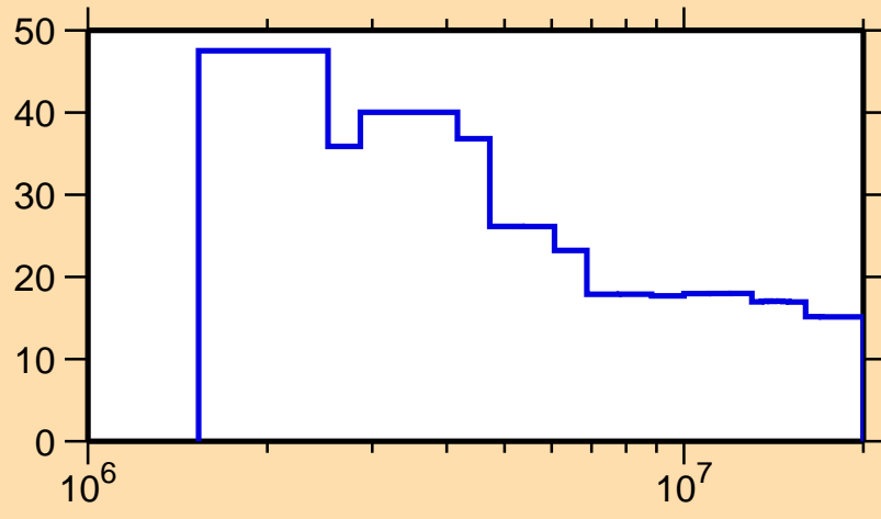
\Delta\sigma/\sigma vs. E for ^{50}\text{Mn}(n,n\text{cont.})
