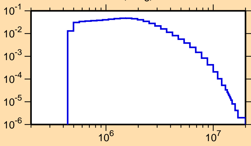
\sigma vs. E for ^{50}\text{Mn}(n,n_3)
