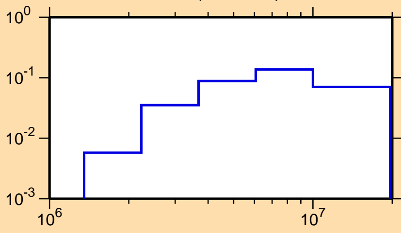
\sigma vs. E for ^{50}\text{Mn}(n,n\text{cont.})
