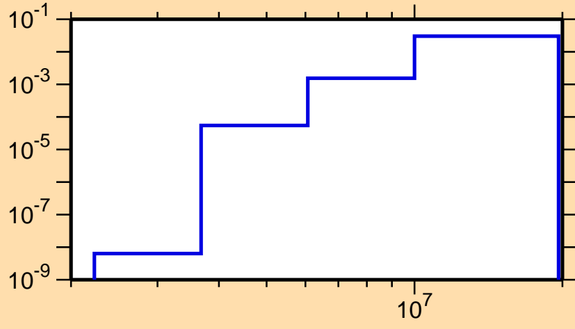
\sigma vs. E for ^{50}\text{Mn}(n,d)
