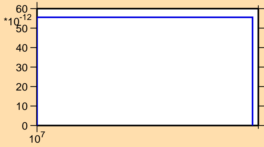
\sigma vs. E for ^{50}\text{Mn} (mt 45)
