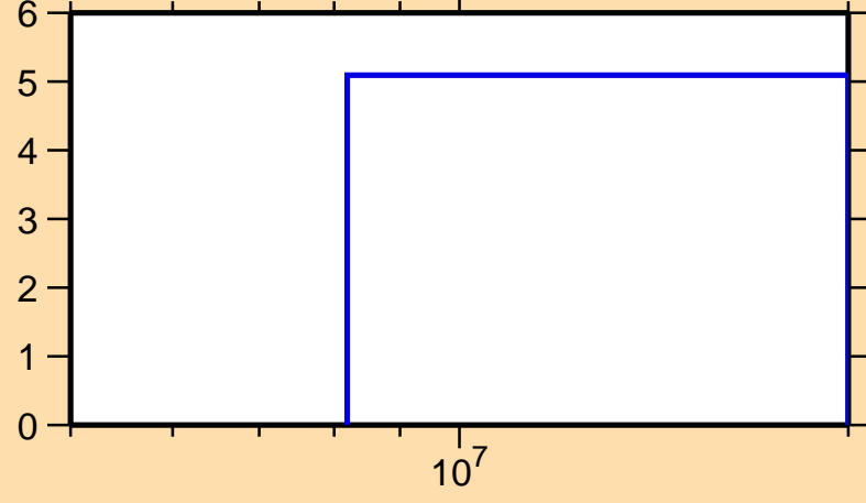
\Delta\sigma/\sigma vs. E for ^{50}\text{Mn}(n,\text{el.})
