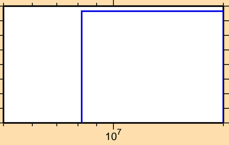
\sigma vs. E for ^{50}\text{Mn}(n,n\alpha)
