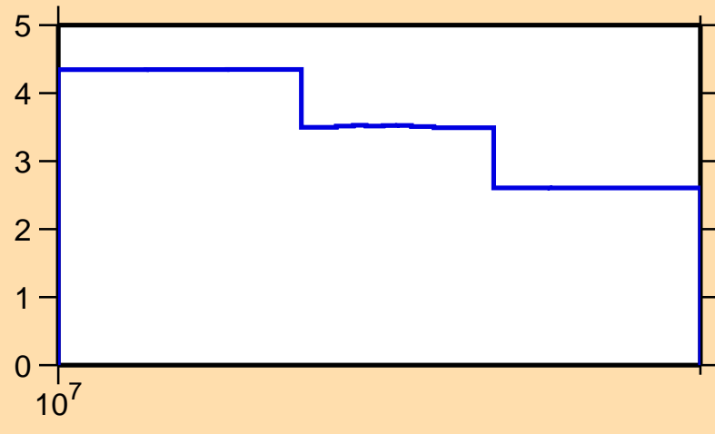
\Delta\sigma/\sigma vs. E for ^{52}\text{Mn}(n,\text{el.})
