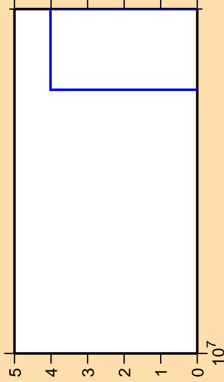
\Delta\sigma/\sigma vs. E for ^{52}\text{Mn}(n,\text{pt})
