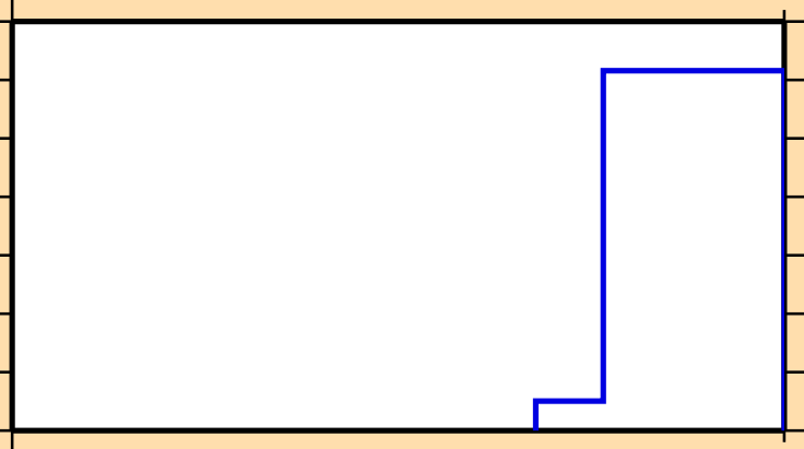
\sigma vs. E for ^{52}\text{Mn}(\text{mt117})
