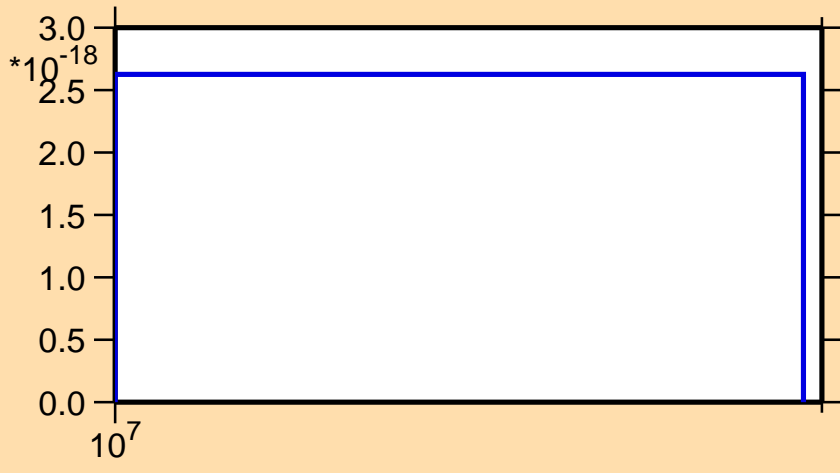
\sigma vs. E for ^{52}\text{Mn} (mt 34)
