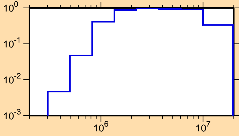
\sigma vs. E for ^{52}\text{Mn}(n,\text{inel.})
