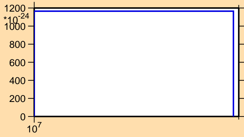
\sigma vs. E for ^{52}\text{Mn}(n,2n\alpha)
