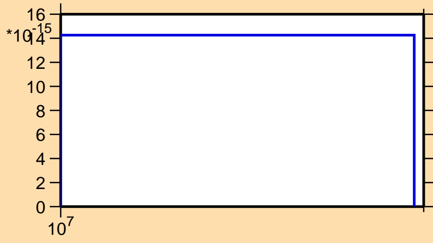
\sigma vs. E for ^{52}\text{Mn}(n,\text{pt})
