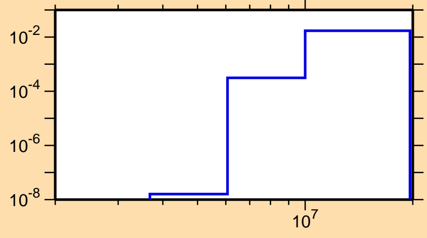
\sigma vs. E for ^{52}\text{Mn}(n,d)
