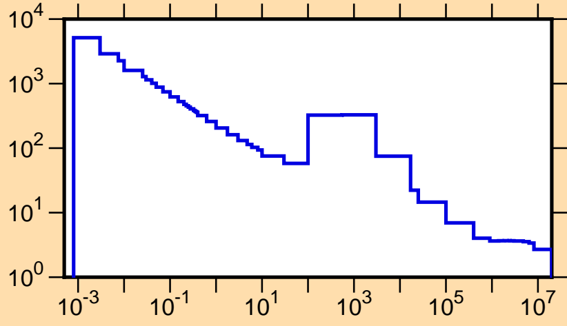
\sigma vs. E for ^{52}\text{Mn}(n,\text{tot.})
