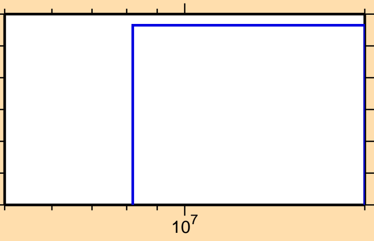
\sigma vs. E for ^{52}\text{Mn}(n,2np)
