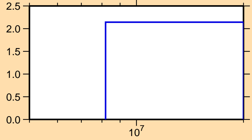
\Delta\sigma/\sigma vs. E for ^{52}\text{Mn}(n,\text{nonel.})
