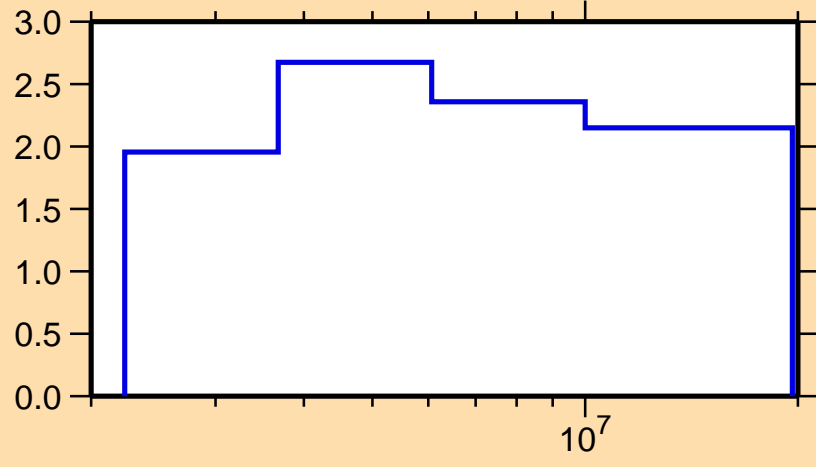
\Delta\sigma/\sigma vs. E for ^{52}\text{Mn}(n,n\text{inel.})
