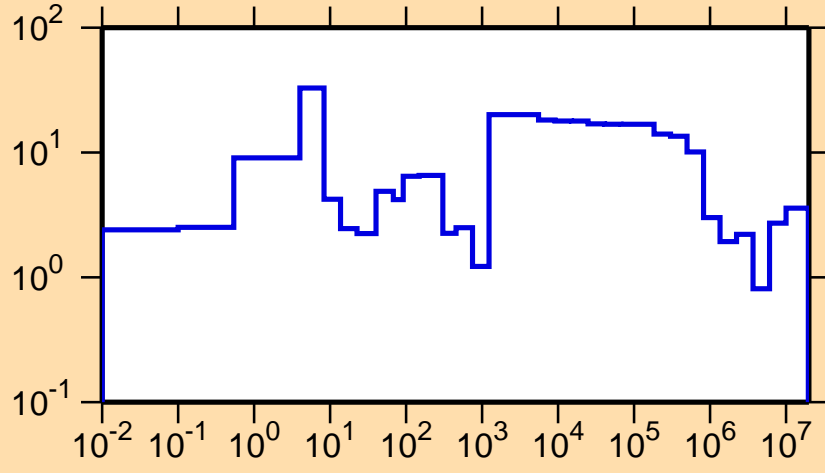
\Delta\sigma/\sigma vs. E for ^{52}\text{Mn}(n,el.)
