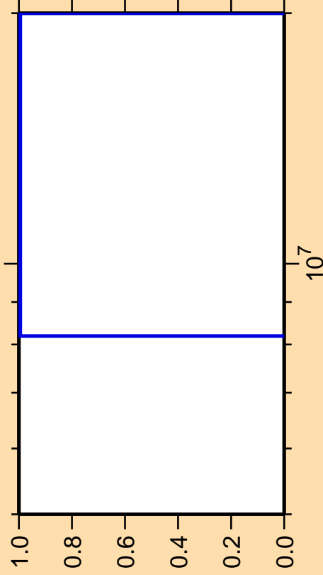
\Delta\sigma/\sigma vs. E for ^{52}\text{Mn}(n,pt)
