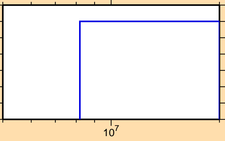
\sigma vs. E for ^{52}\text{Mn}(n,nd)
