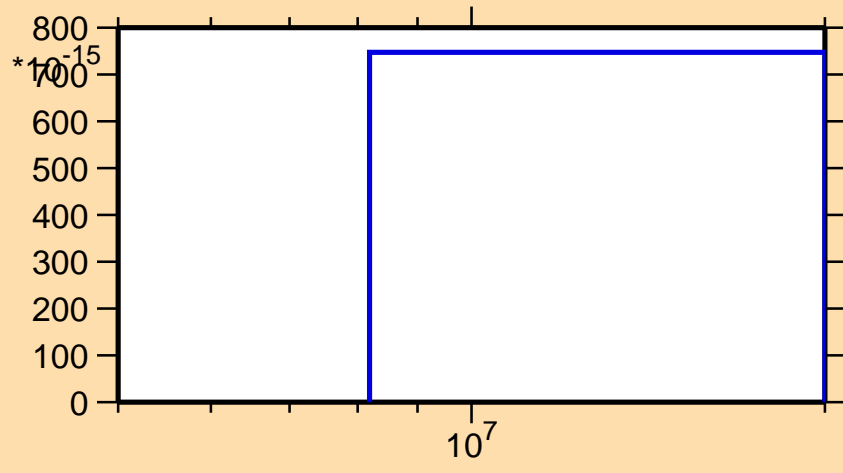
\sigma vs. E for ^{52}\text{Mn}(n,pt)
