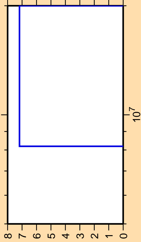
\Delta\sigma/\sigma vs. E for ^{52}\text{Mn}(n,p)
