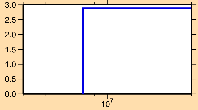
\Delta\sigma/\sigma vs. E for ^{53}\text{Mn}(n,\text{nonel.})
