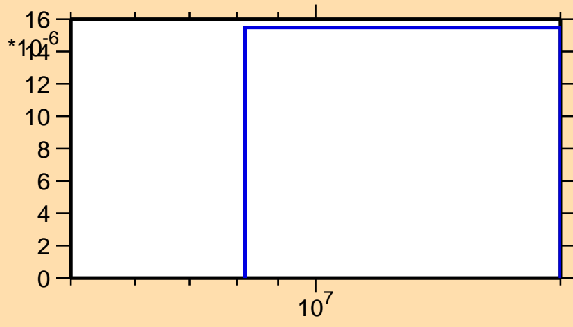
\sigma vs. E for ^{53}\text{Mn}(n,p\alpha)
