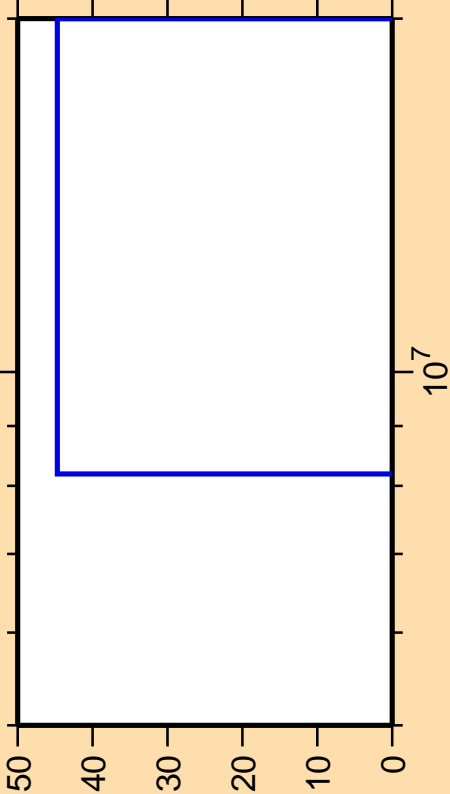
\Delta\sigma/\sigma vs. E for ^{53}\text{Mn}(n,pd)
