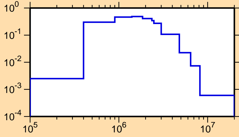
\sigma vs. E for ^{53}\text{Mn}(n,n_1)
