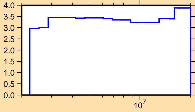
\Delta\sigma/\sigma vs. E for ^{54}\text{Mn}(n,n\text{onel.})
