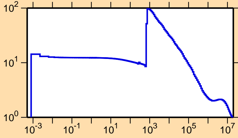
\sigma vs. E for ^{54}\text{Mn}(n,\text{el.})
