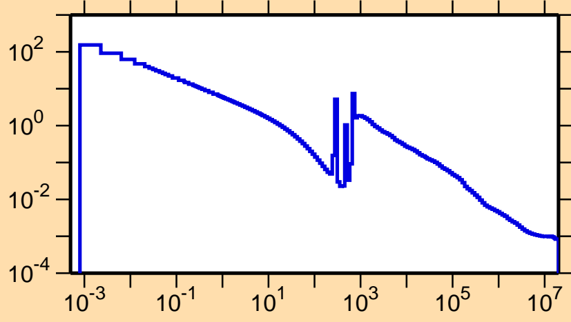
\sigma vs. E for ^{54}\text{Mn}(n,\gamma)
