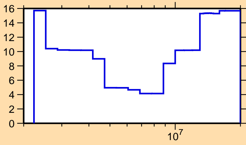
\Delta\sigma/\sigma vs. E for ^{54}\text{Mn}(n,n\text{cont.})
