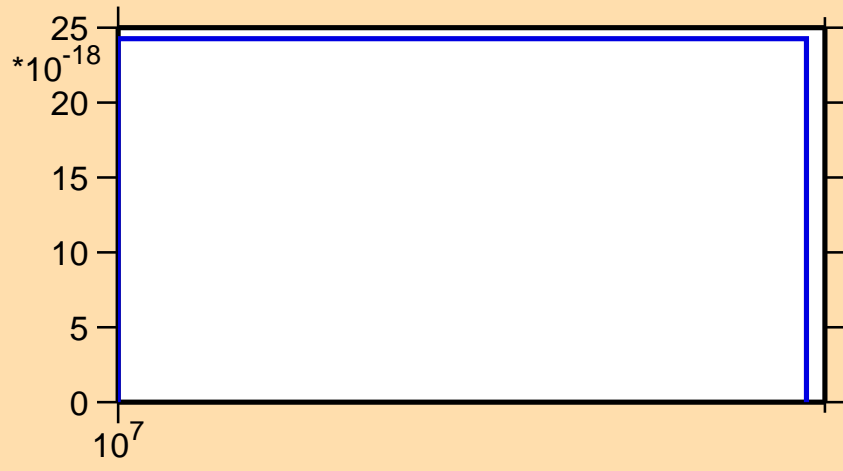
\sigma vs. E for ^{54}\text{Mn} (mt 34)
