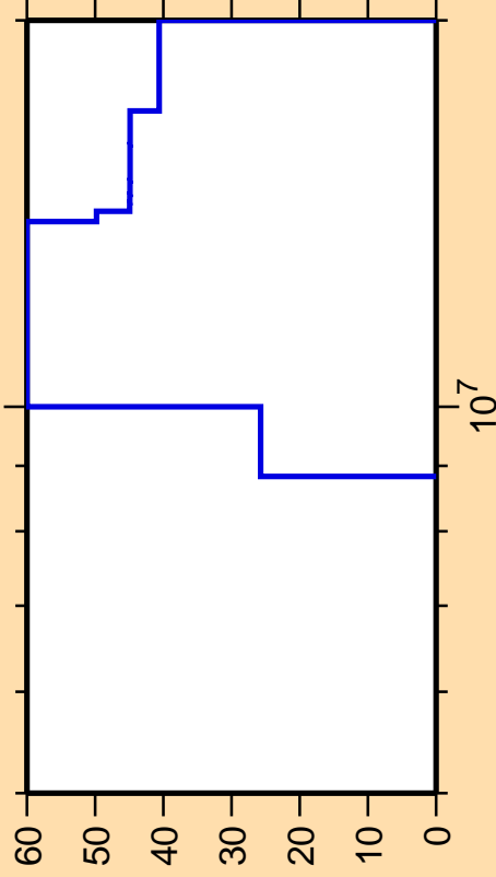
\Delta\sigma/\sigma vs. E for ^{56}\text{Mn}(n,np)
