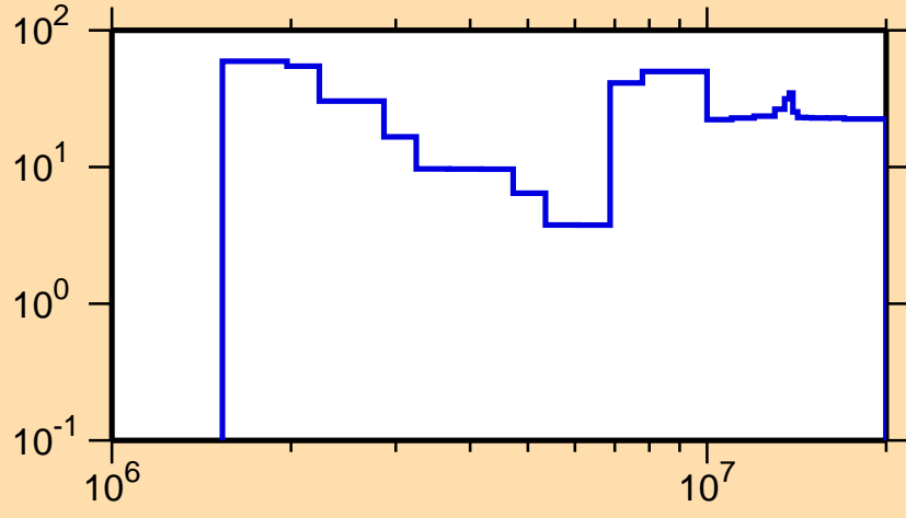
\Delta\sigma/\sigma vs. E for ^{56}\text{Mn}(n,n\text{cont.})
