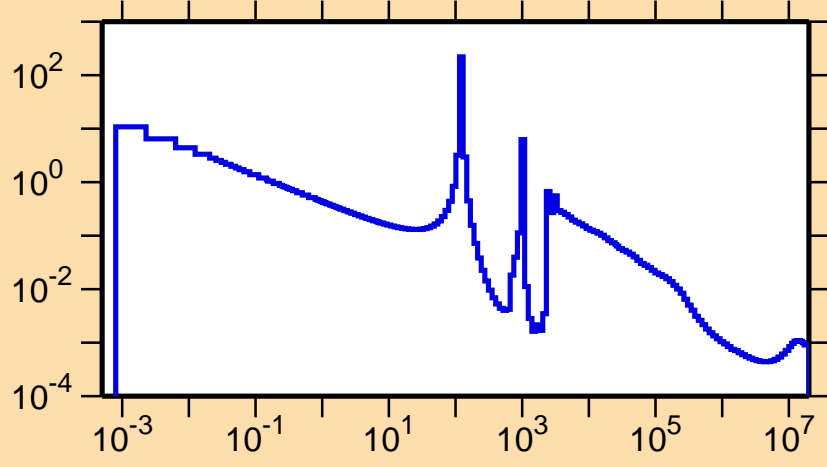
\sigma vs. E for ^{56}\text{Mn}(n,\gamma)
