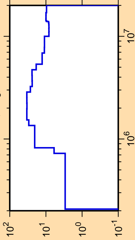
\Delta\sigma/\sigma vs. E for ^{56}\text{Mn}(n,n_3)
