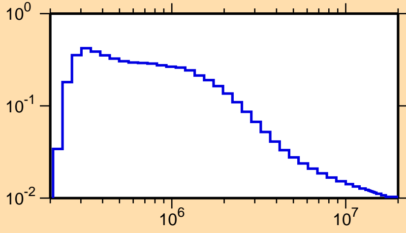
\sigma vs. E for ^{56}\text{Mn}(n,n_3)
