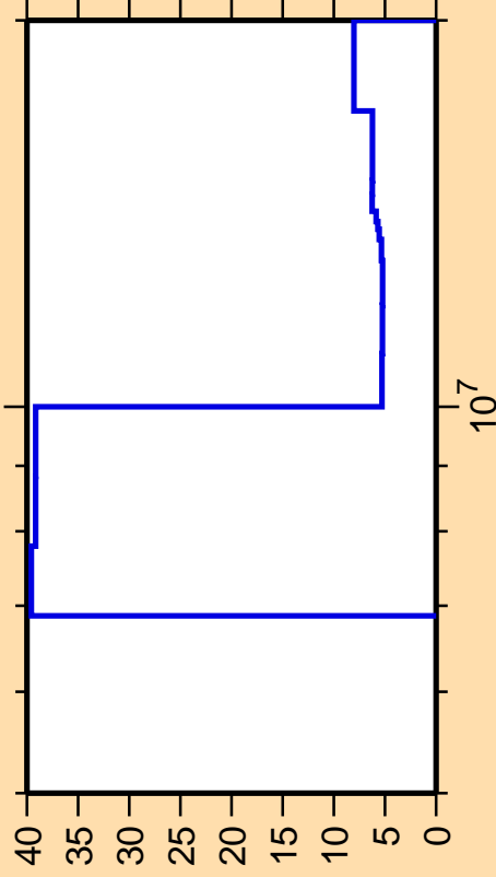
\Delta\sigma/\sigma vs. E for ^{56}\text{Mn}(n,2n)
