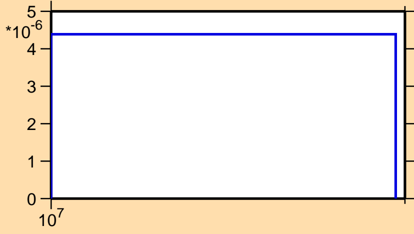
\sigma vs. E for ^{56}\text{Mn}(n,nd)
