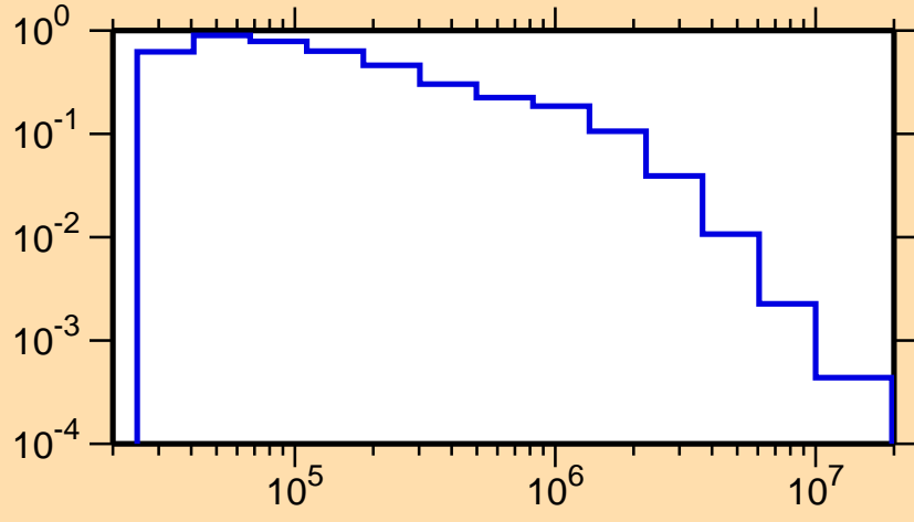
\sigma vs. E for ^{56}\text{Mn}(n,n_1)
