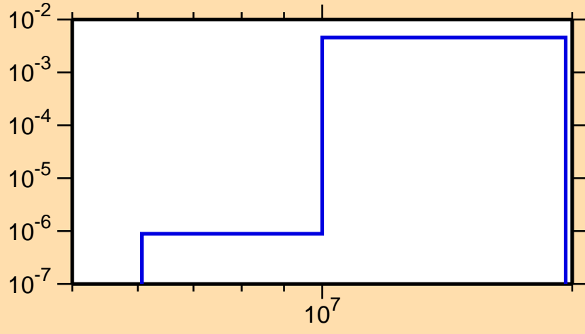
\sigma vs. E for ^{56}\text{Mn}(n,d)
