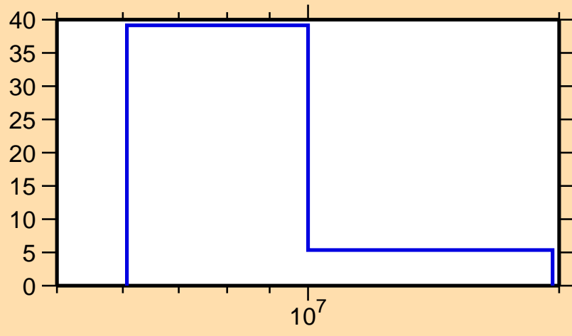
\Delta\sigma/\sigma vs. E for ^{56}\text{Mn}(n,2n)
