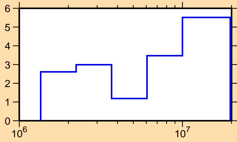
\Delta\sigma/\sigma vs. E for ^{56}\text{Mn}(n,\text{tot.})
