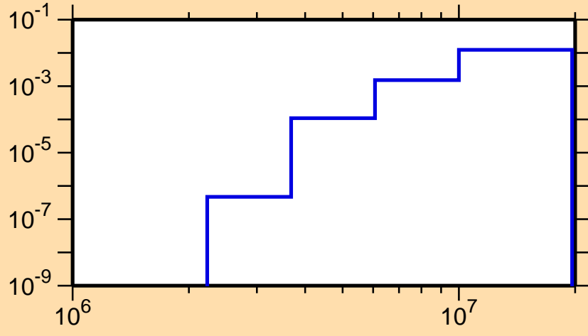
\sigma vs. E for ^{56}\text{Mn}(n,\alpha)
