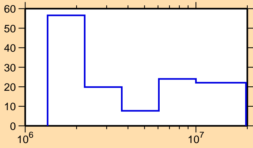
\Delta\sigma/\sigma vs. E for ^{56}\text{Mn}(n,n\text{cont.})
