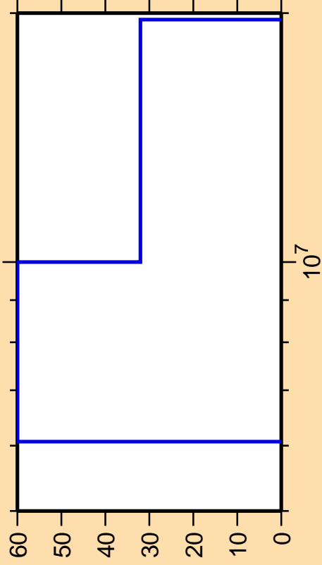
\Delta\sigma/\sigma vs. E for ^{56}\text{Mn}(n,d)
