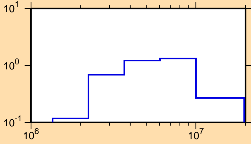
\sigma vs. E for ^{56}\text{Mn}(n,n\text{cont.})
