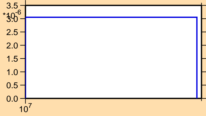
\sigma vs. E for ^{56}\text{Mn}(n,2np)
