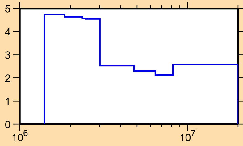
\Delta\sigma/\sigma vs. E for ^{56}\text{Mn}(n,n\text{nonel.})
