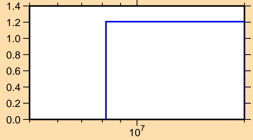
\Delta\sigma/\sigma vs. E for ^{57}\text{Mn}(n,\text{nonel.})
