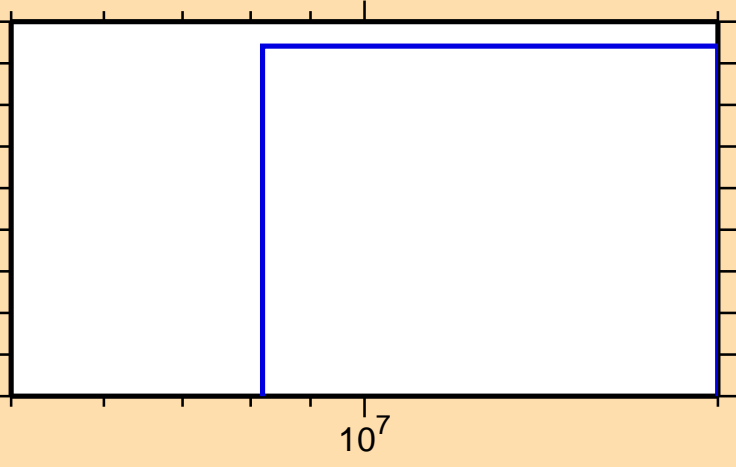
\sigma vs. E for ^{57}\text{Mn}(n,np)
