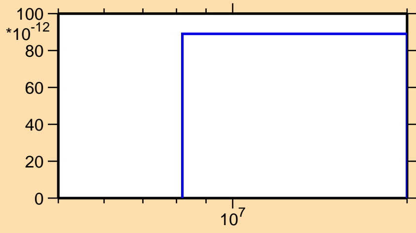
\sigma vs. E for ^{58}\text{Mn}(n,2n\alpha)
