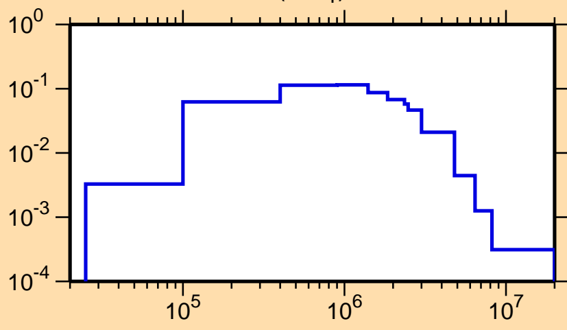
\sigma vs. E for ^{58}\text{Mn}(n,n_1)
