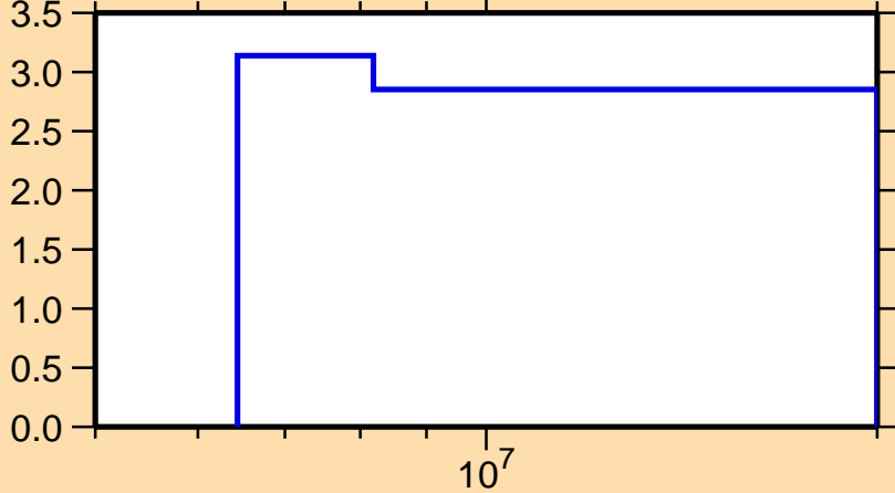
\Delta\sigma/\sigma vs. E for ^{58}\text{Mn}(n,\text{nonel.})
