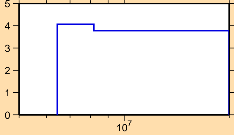
\Delta\sigma/\sigma vs. E for ^{58}\text{Mn}(n,2n)
