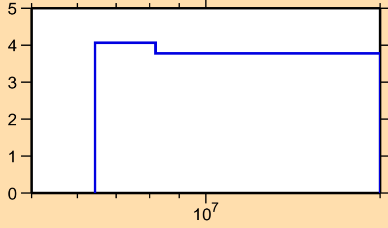
\Delta\sigma/\sigma vs. E for ^{58}\text{Mn}(n,2n)
